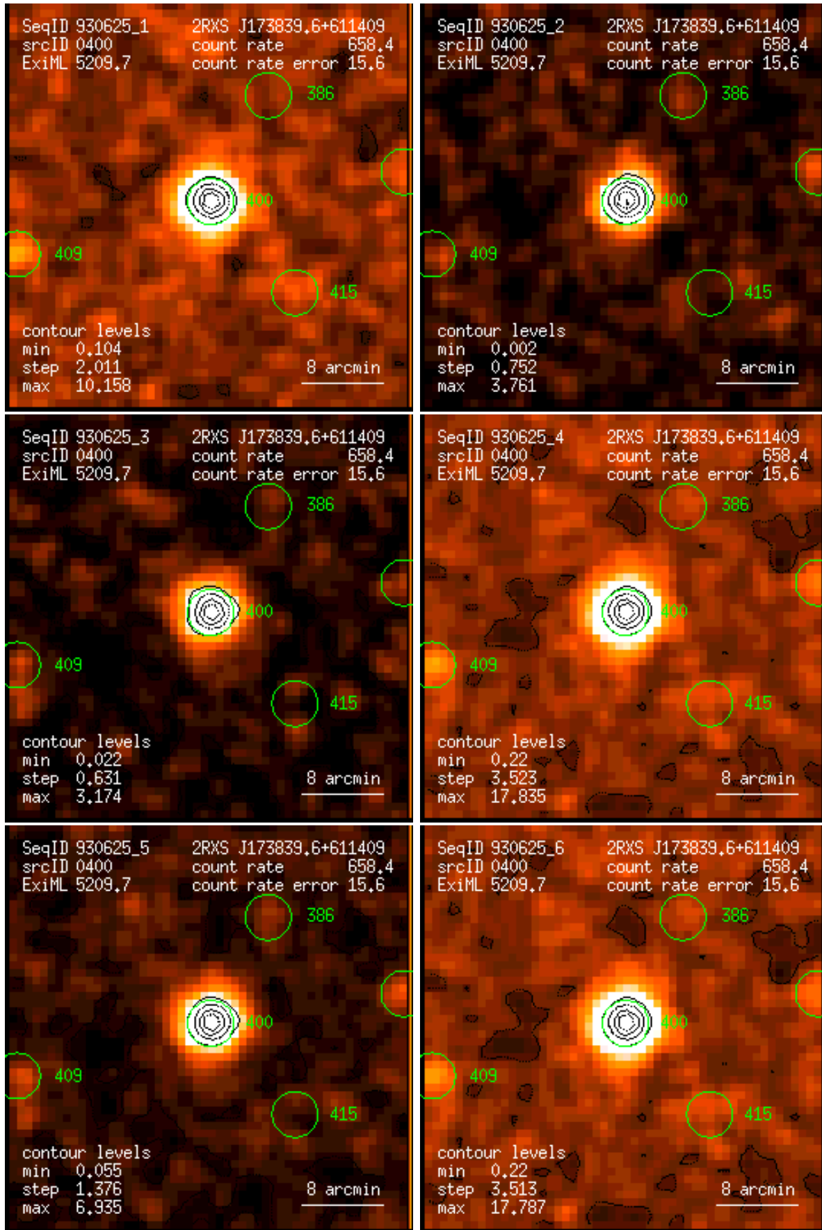
Figure 400: RASS 930625: detection 0400: band rate images, Gaussian filter: (1) PSPC channels 11 – 41, (2) 52 – 90, (3) 91 – 201, (4) 11 – 235, (5) 52 – 201, (6) 11 – 201. Broad band rates in counts/ks. Band rate contour levels in counts/ks/arcmin 2 .
