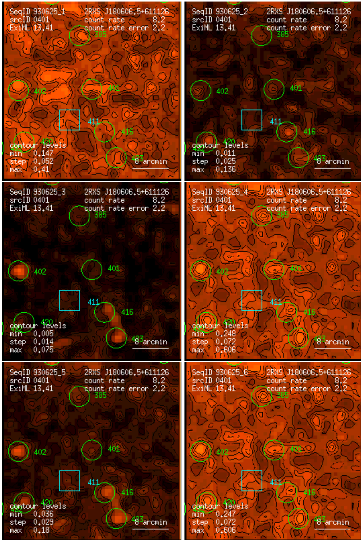
Figure 401: RASS 930625: detection 0401: band rate images, Gaussian filter: (1) PSPC channels 11 – 41, (2) 52 – 90, (3) 91 – 201, (4) 11 – 235, (5) 52 – 201, (6) 11 – 201. Broad band rates in counts/ks. Band rate contour levels in counts/ks/arcmin 2 .
