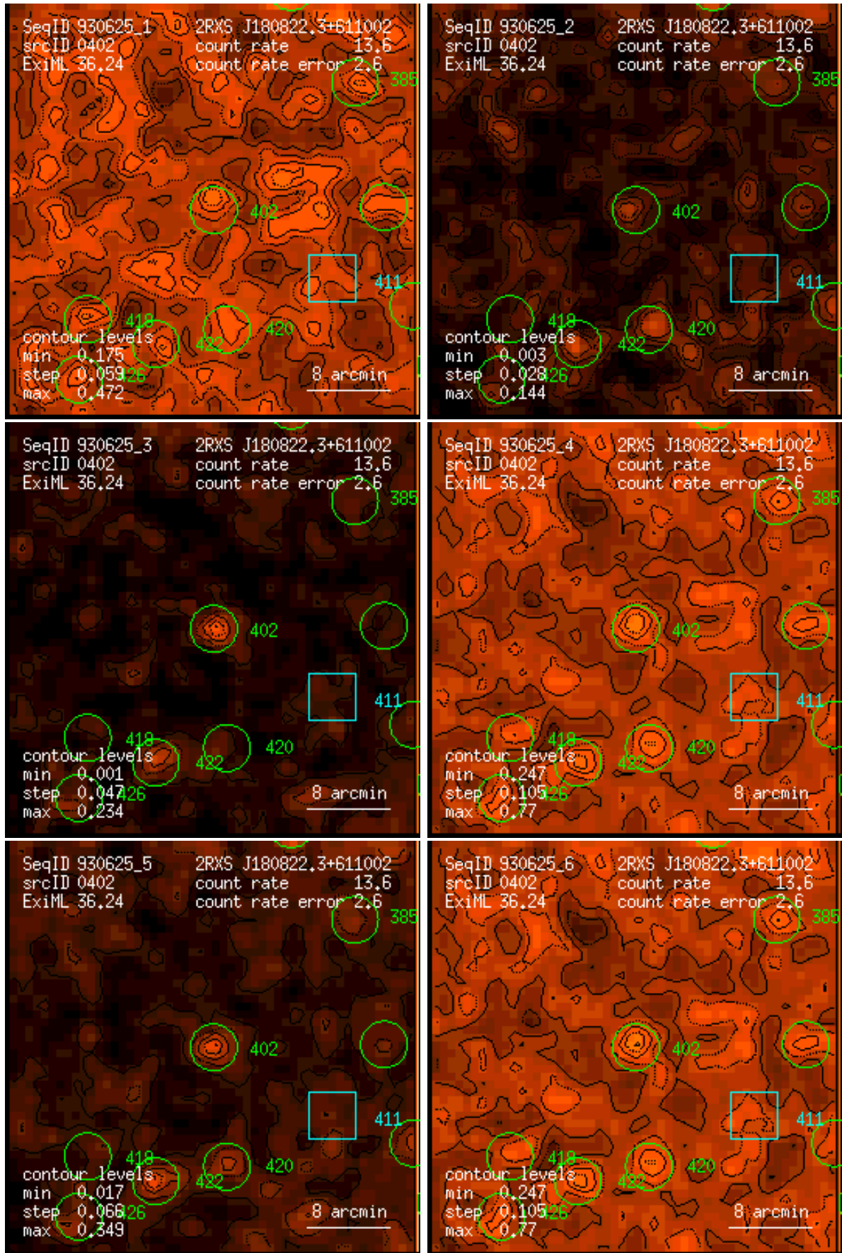
Figure 402: RASS 930625: detection 0402: band rate images, Gaussian filter: (1) PSPC channels 11 – 41, (2) 52 – 90, (3) 91 – 201, (4) 11 – 235, (5) 52 – 201, (6) 11 – 201. Broad band rates in counts/ks. Band rate contour levels in counts/ks/arcmin 2 .
