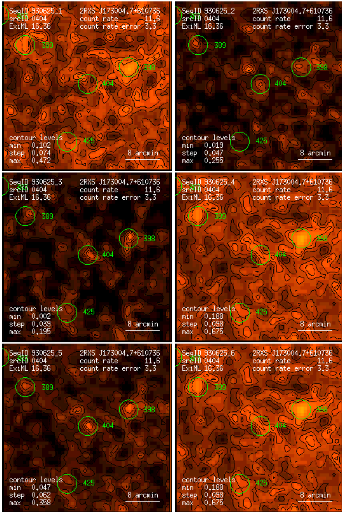
Figure 404: RASS 930625: detection 0404: band rate images, Gaussian filter: (1) PSPC channels 11 – 41, (2) 52 – 90, (3) 91 – 201, (4) 11 – 235, (5) 52 – 201, (6) 11 – 201. Broad band rates in counts/ks. Band rate contour levels in counts/ks/arcmin 2 .
