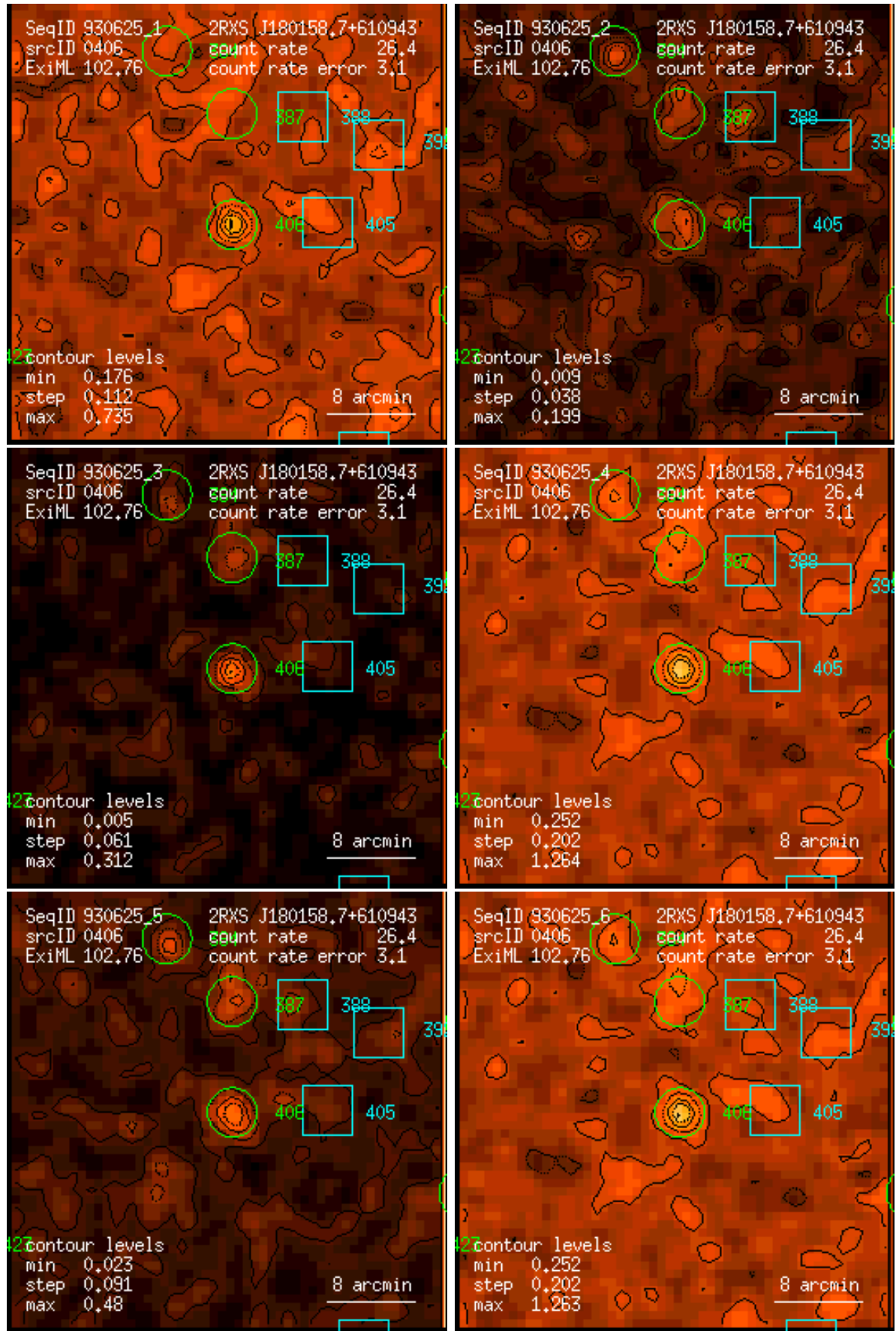
Figure 406: RASS 930625: detection 0406: band rate images, Gaussian filter: (1) PSPC channels 11 – 41, (2) 52 – 90, (3) 91 – 201, (4) 11 – 235, (5) 52 – 201, (6) 11 – 201. Broad band rates in counts/ks. Band rate contour levels in counts/ks/arcmin 2 .
