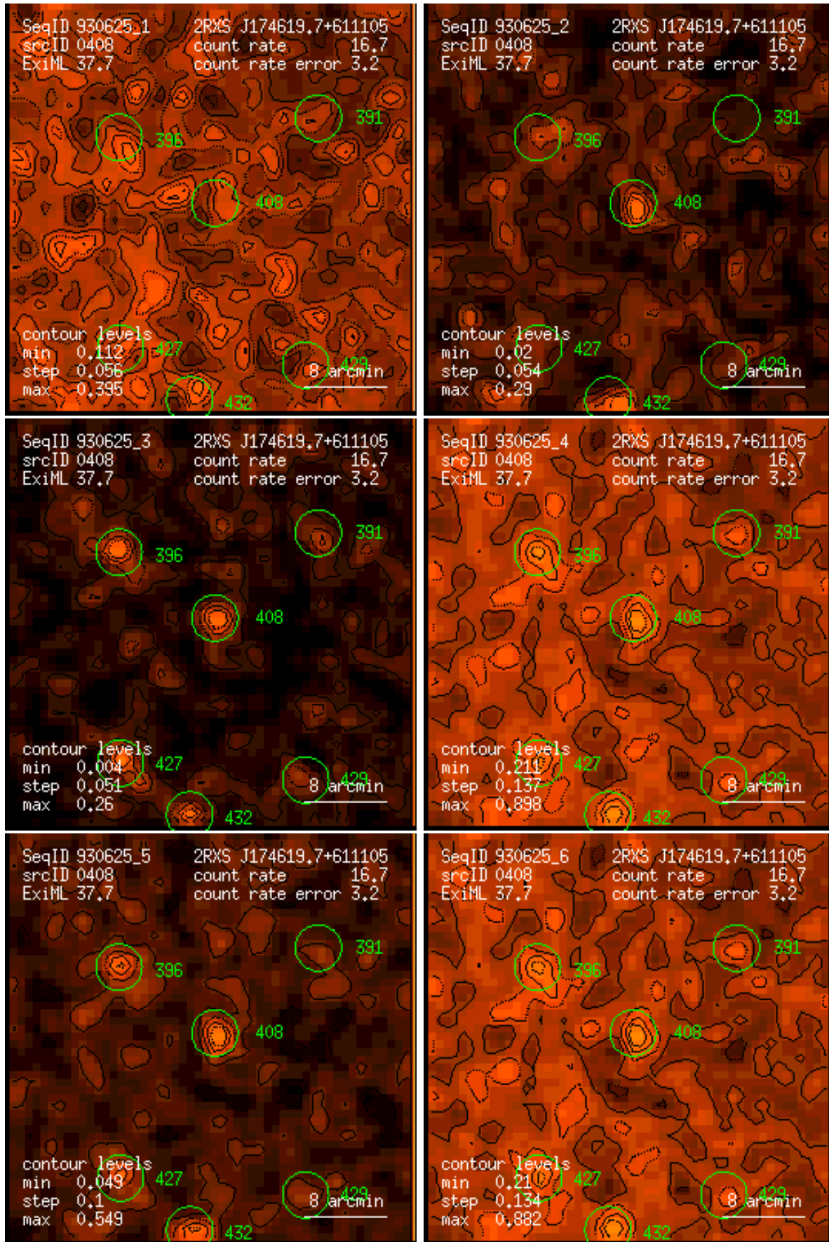
Figure 408: RASS 930625: detection 0408: band rate images, Gaussian filter: (1) PSPC channels 11 – 41, (2) 52 – 90, (3) 91 – 201, (4) 11 – 235, (5) 52 – 201, (6) 11 – 201. Broad band rates in counts/ks. Band rate contour levels in counts/ks/arcmin 2 .
