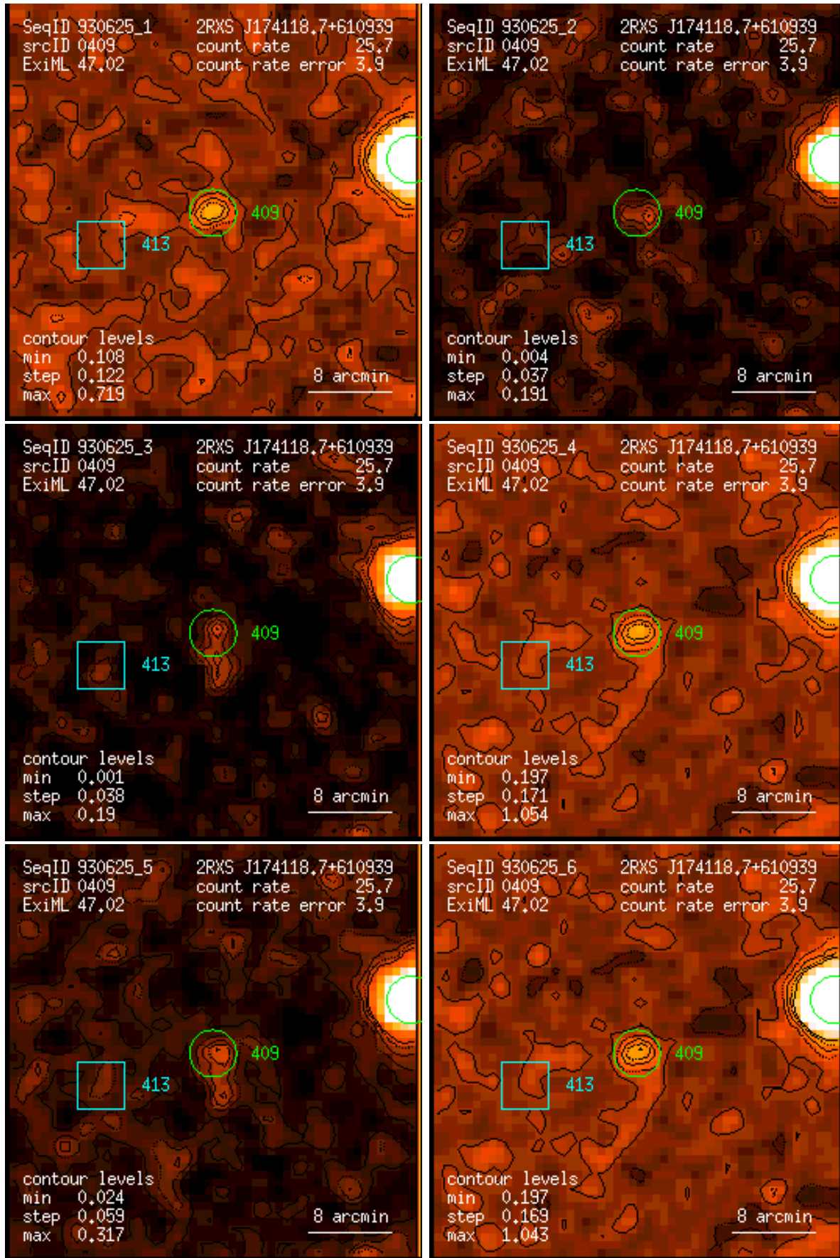
Figure 409: RASS 930625: detection 0409: band rate images, Gaussian filter: (1) PSPC channels 11 – 41, (2) 52 – 90, (3) 91 – 201, (4) 11 – 235, (5) 52 – 201, (6) 11 – 201. Broad band rates in counts/ks. Band rate contour levels in counts/ks/arcmin 2 .
