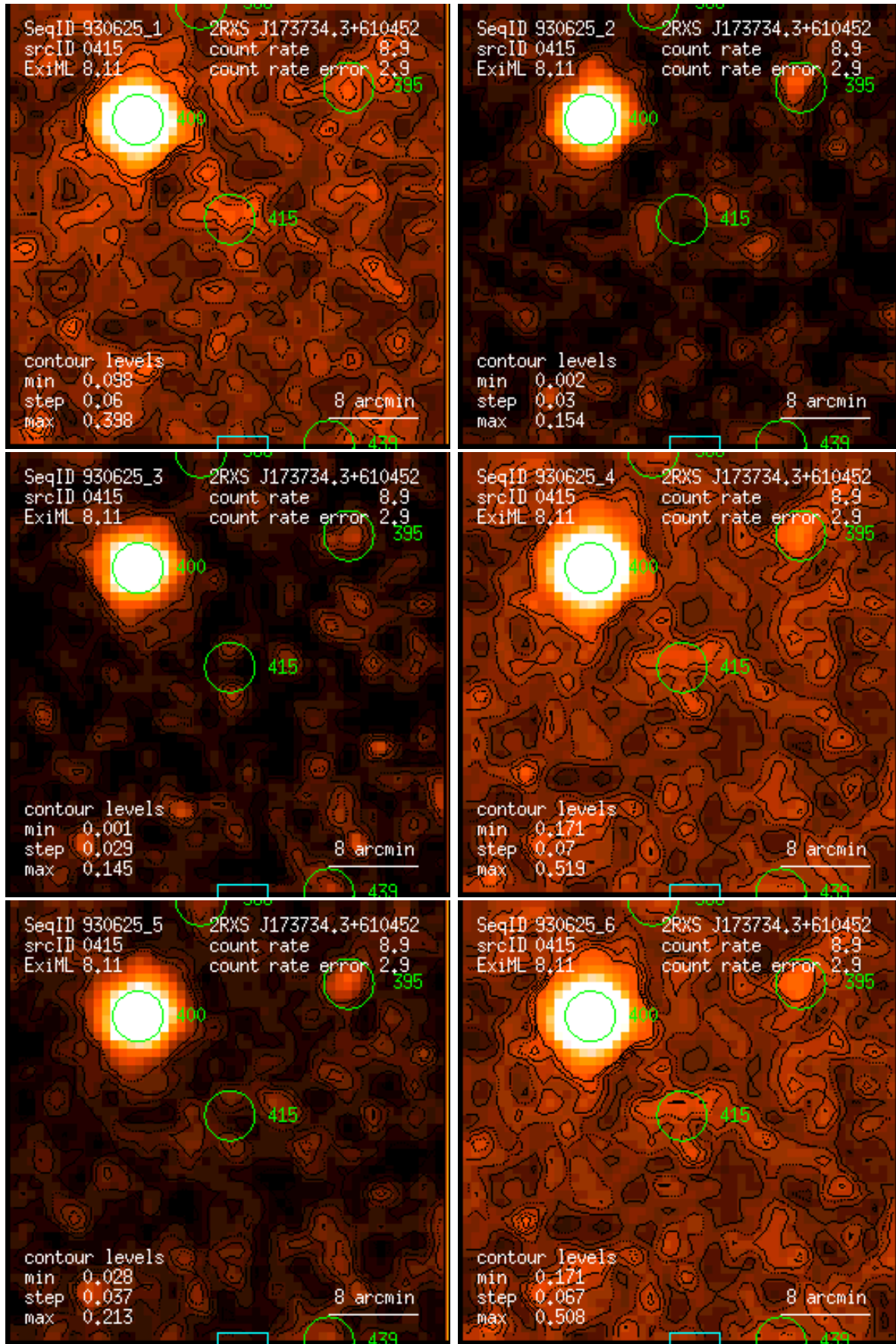
Figure 415: RASS 930625: detection 0415: band rate images, Gaussian filter: (1) PSPC channels 11 – 41, (2) 52 – 90, (3) 91 – 201, (4) 11 – 235, (5) 52 – 201, (6) 11 – 201. Broad band rates in counts/ks. Band rate contour levels in counts/ks/arcmin 2 .
