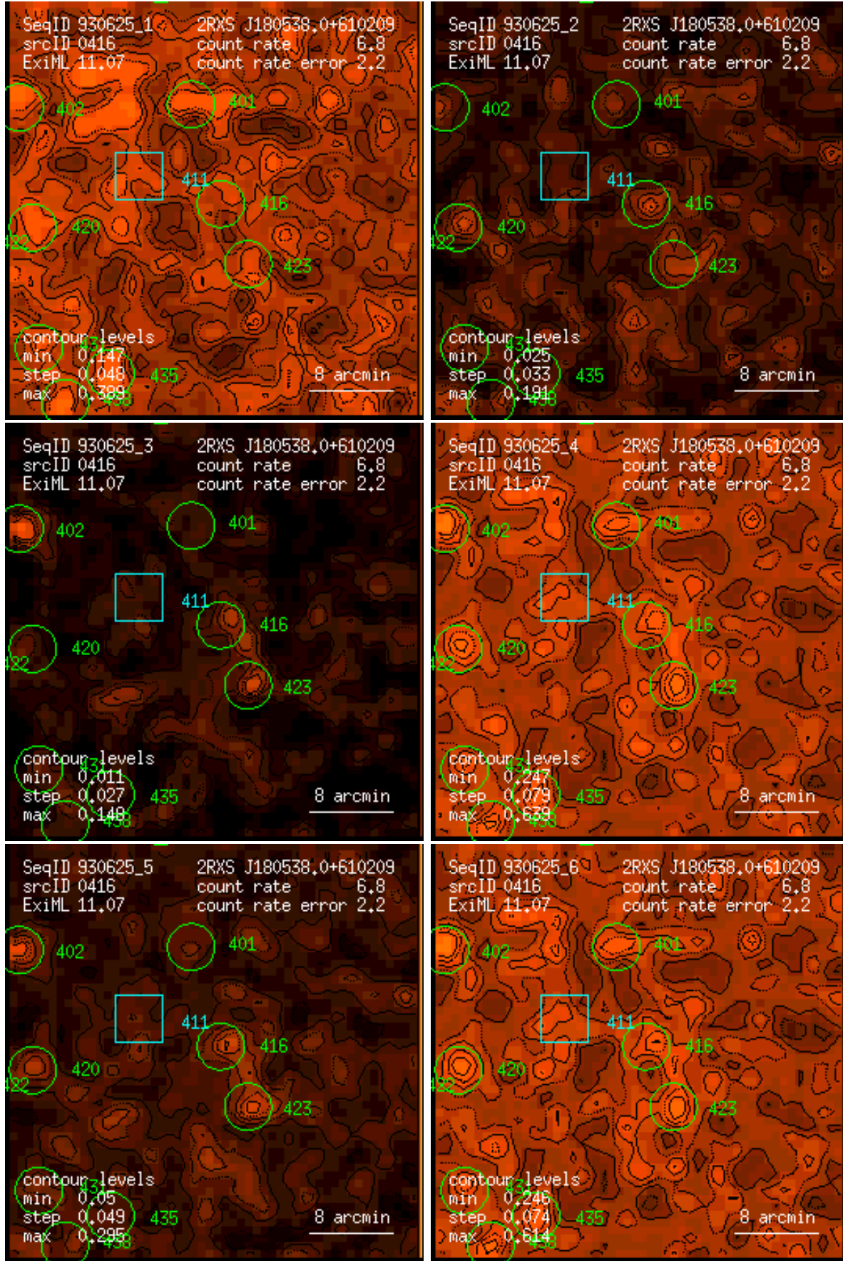
Figure 416: RASS 930625: detection 0416: band rate images, Gaussian filter: (1) PSPC channels 11 – 41, (2) 52 – 90, (3) 91 – 201, (4) 11 – 235, (5) 52 – 201, (6) 11 – 201. Broad band rates in counts/ks. Band rate contour levels in counts/ks/arcmin 2 .
