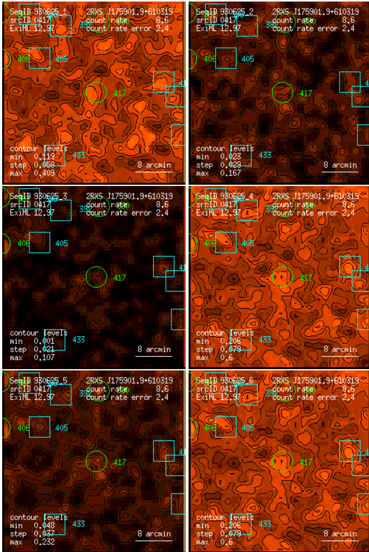
Figure 417: RASS 930625: detection 0417: band rate images, Gaussian filter: (1) PSPC channels 11 – 41, (2) 52 – 90, (3) 91 – 201, (4) 11 – 235, (5) 52 – 201, (6) 11 – 201. Broad band rates in counts/ks. Band rate contour levels in counts/ks/arcmin 2 .
