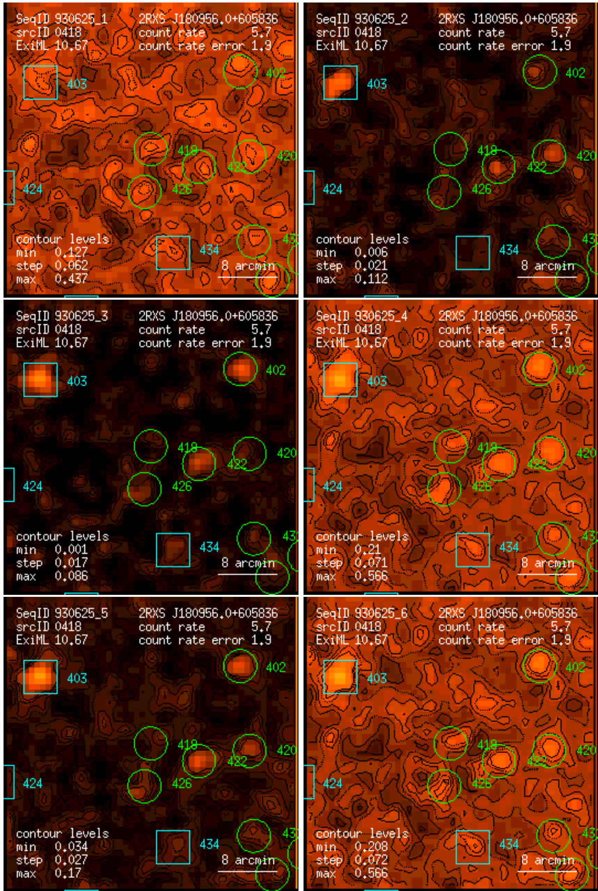
Figure 418: RASS 930625: detection 0418: band rate images, Gaussian filter: (1) PSPC channels 11 – 41, (2) 52 – 90, (3) 91 – 201, (4) 11 – 235, (5) 52 – 201, (6) 11 – 201. Broad band rates in counts/ks. Band rate contour levels in counts/ks/arcmin 2 .
