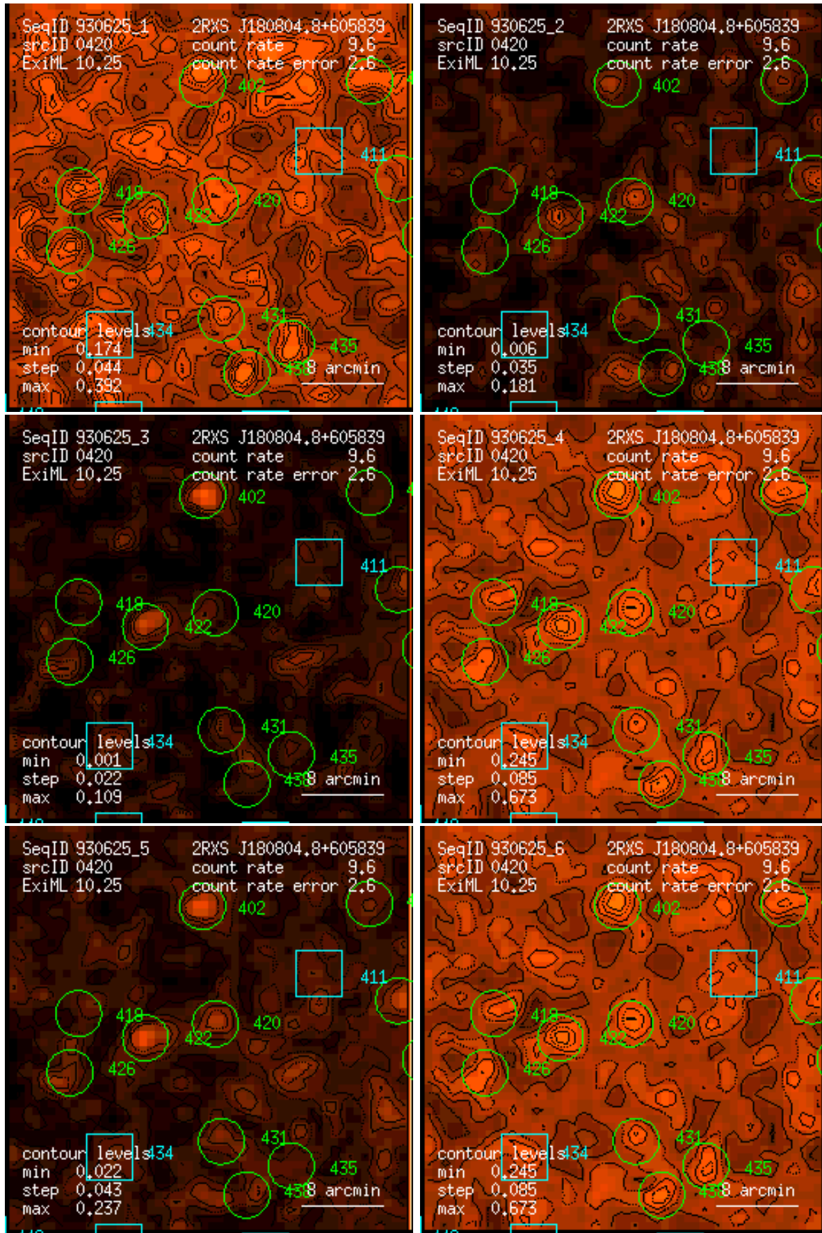
Figure 420: RASS 930625: detection 0420: band rate images, Gaussian filter: (1) PSPC channels 11 – 41, (2) 52 – 90, (3) 91 – 201, (4) 11 – 235, (5) 52 – 201, (6) 11 – 201. Broad band rates in counts/ks. Band rate contour levels in counts/ks/arcmin 2 .
