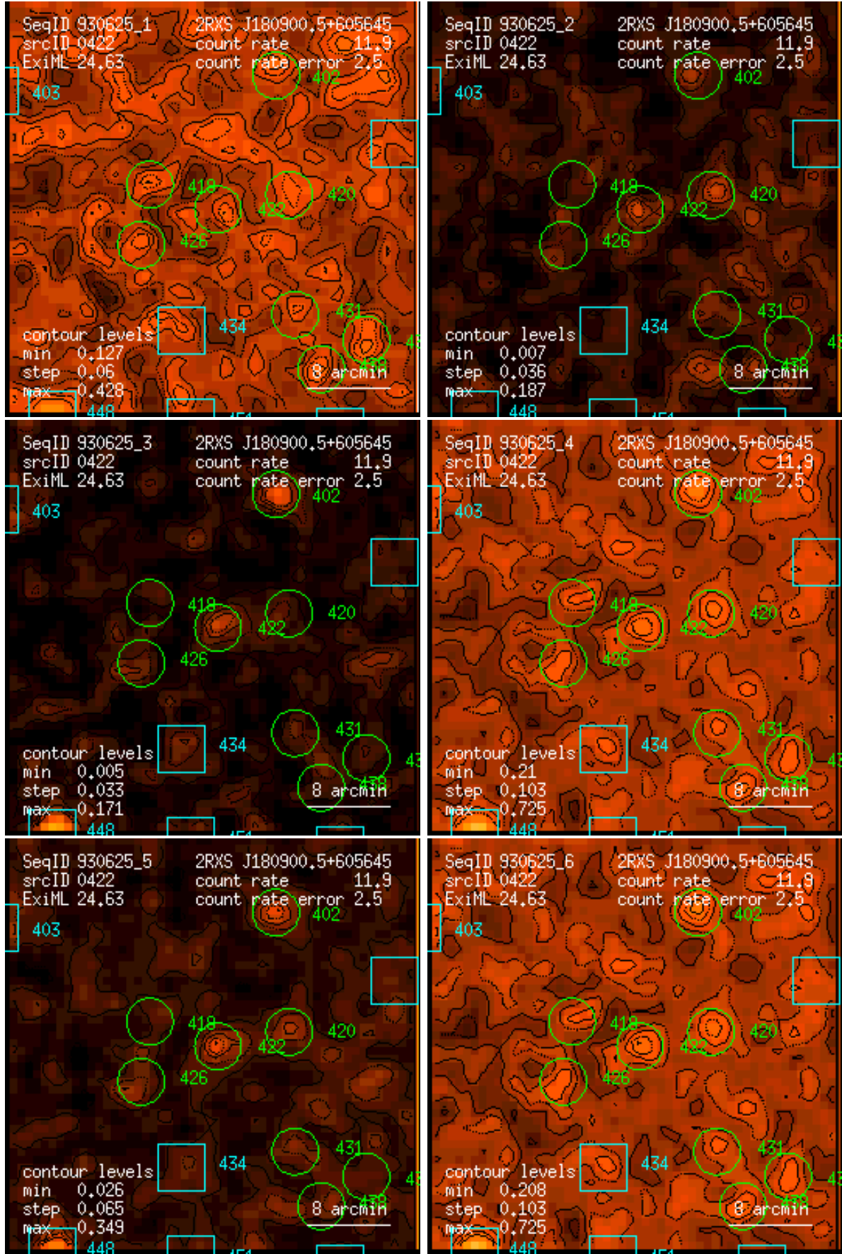
Figure 422: RASS 930625: detection 0422: band rate images, Gaussian filter: (1) PSPC channels 11 – 41, (2) 52 – 90, (3) 91 – 201, (4) 11 – 235, (5) 52 – 201, (6) 11 – 201. Broad band rates in counts/ks. Band rate contour levels in counts/ks/arcmin 2 .
