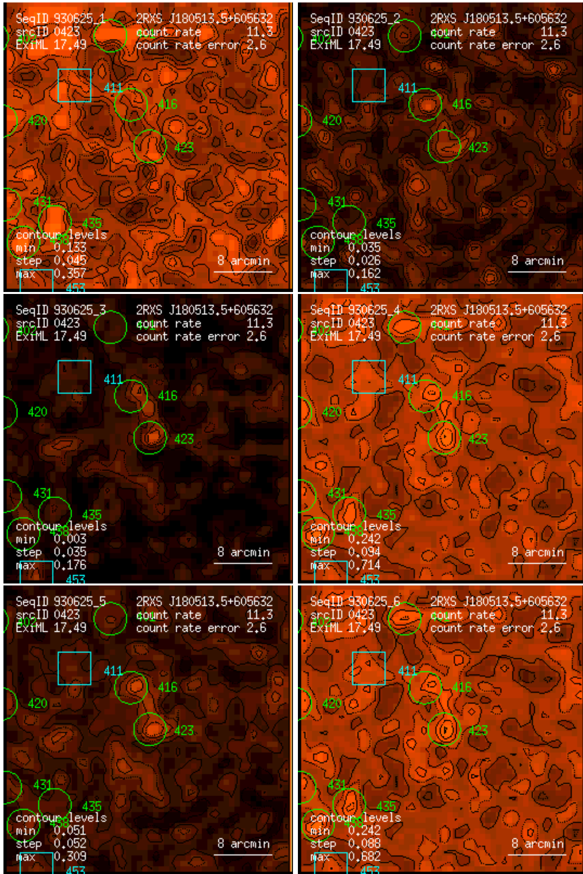
Figure 423: RASS 930625: detection 0423: band rate images, Gaussian filter: (1) PSPC channels 11 – 41, (2) 52 – 90, (3) 91 – 201, (4) 11 – 235, (5) 52 – 201, (6) 11 – 201. Broad band rates in counts/ks. Band rate contour levels in counts/ks/arcmin 2 .
