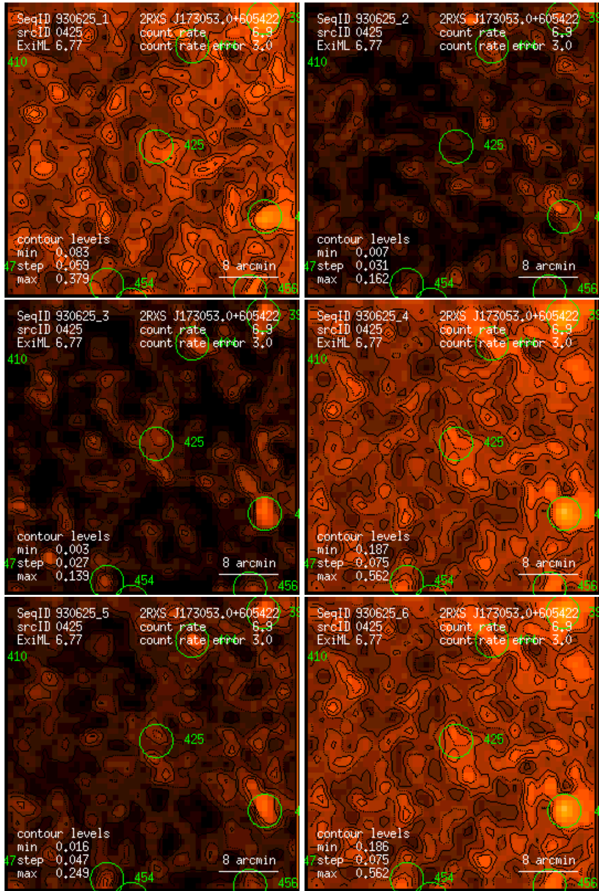
Figure 425: RASS 930625: detection 0425: band rate images, Gaussian filter: (1) PSPC channels 11 – 41, (2) 52 – 90, (3) 91 – 201, (4) 11 – 235, (5) 52 – 201, (6) 11 – 201. Broad band rates in counts/ks. Band rate contour levels in counts/ks/arcmin 2 .
