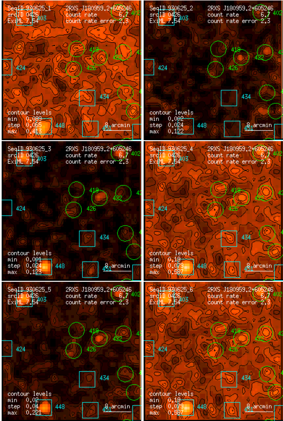
Figure 426: RASS 930625: detection 0426: band rate images, Gaussian filter: (1) PSPC channels 11 – 41, (2) 52 – 90, (3) 91 – 201, (4) 11 – 235, (5) 52 – 201, (6) 11 – 201. Broad band rates in counts/ks. Band rate contour levels in counts/ks/arcmin 2 .
