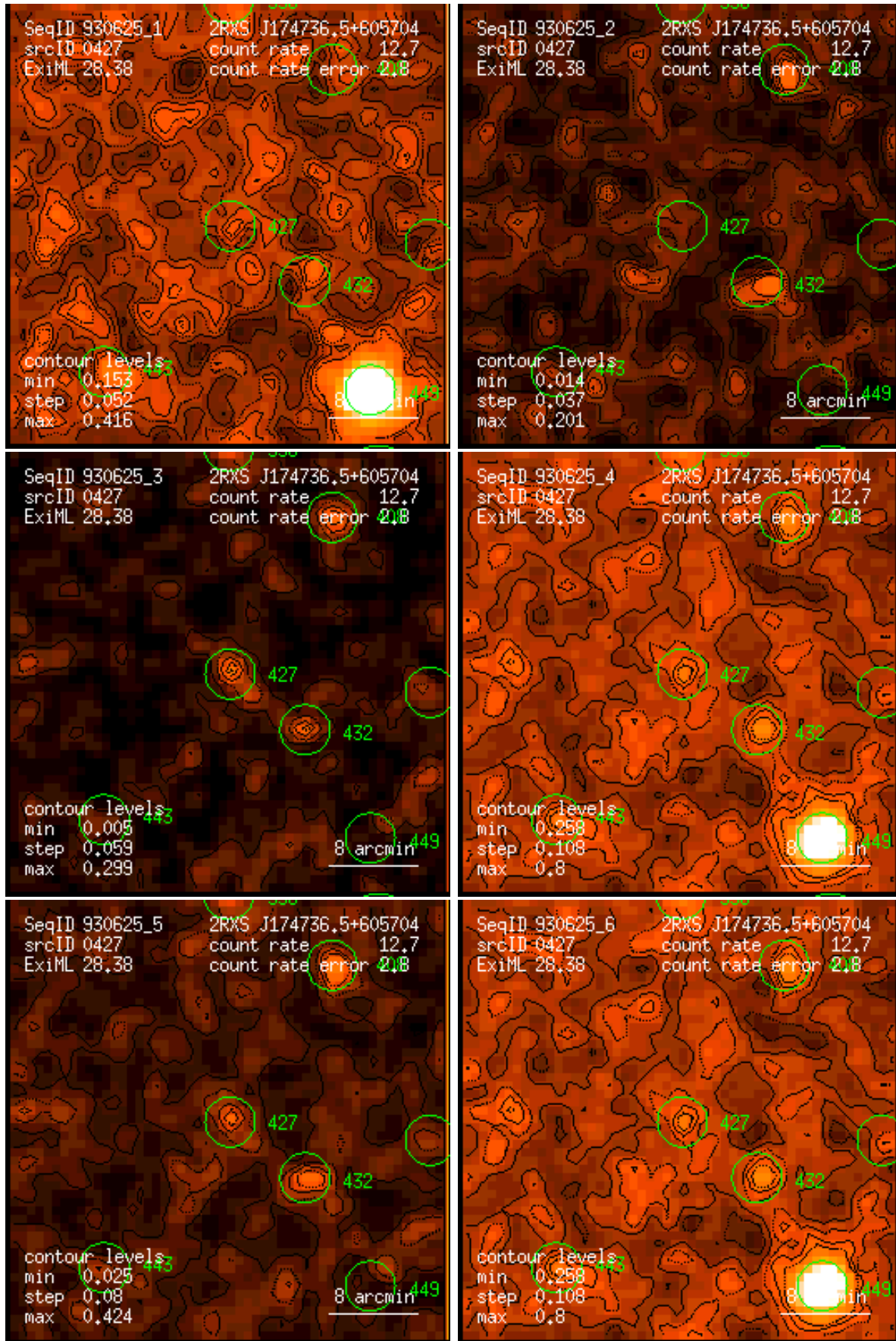
Figure 427: RASS 930625: detection 0427: band rate images, Gaussian filter: (1) PSPC channels 11 – 41, (2) 52 – 90, (3) 91 – 201, (4) 11 – 235, (5) 52 – 201, (6) 11 – 201. Broad band rates in counts/ks. Band rate contour levels in counts/ks/arcmin 2 .
