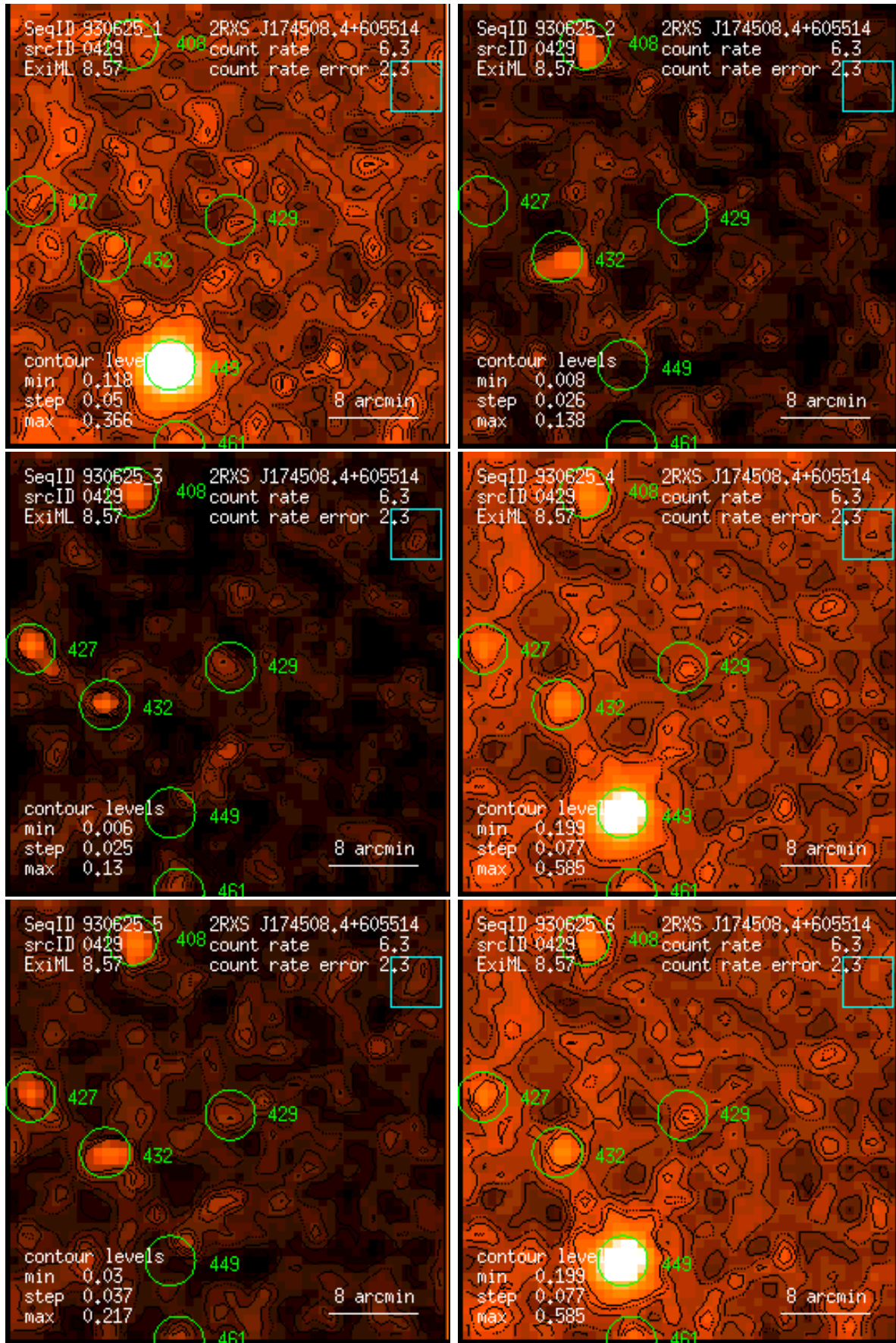
Figure 429: RASS 930625: detection 0429: band rate images, Gaussian filter: (1) PSPC channels 11 – 41, (2) 52 – 90, (3) 91 – 201, (4) 11 – 235, (5) 52 – 201, (6) 11 – 201. Broad band rates in counts/ks. Band rate contour levels in counts/ks/arcmin 2 .
