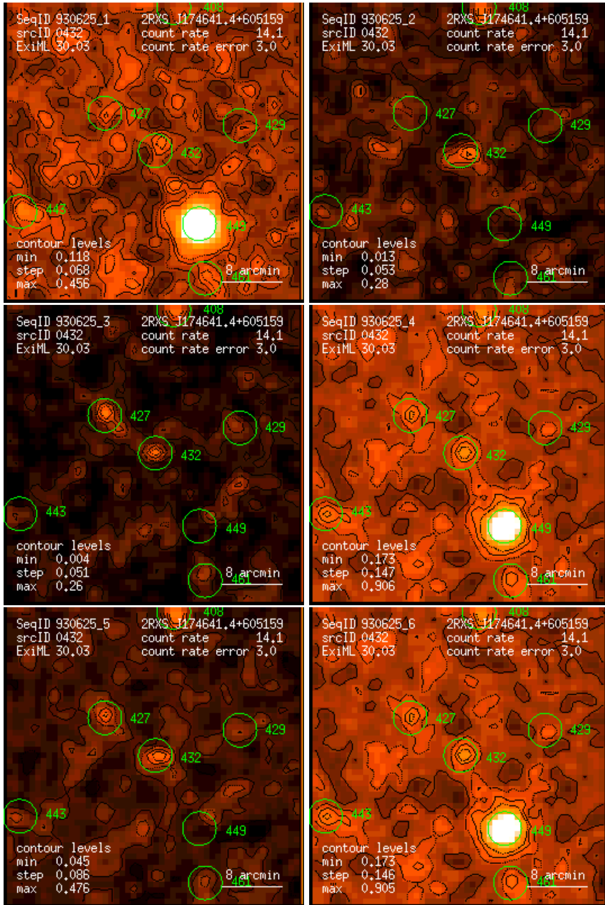
Figure 432: RASS 930625: detection 0432: band rate images, Gaussian filter: (1) PSPC channels 11 – 41, (2) 52 – 90, (3) 91 – 201, (4) 11 – 235, (5) 52 – 201, (6) 11 – 201. Broad band rates in counts/ks. Band rate contour levels in counts/ks/arcmin 2 .
