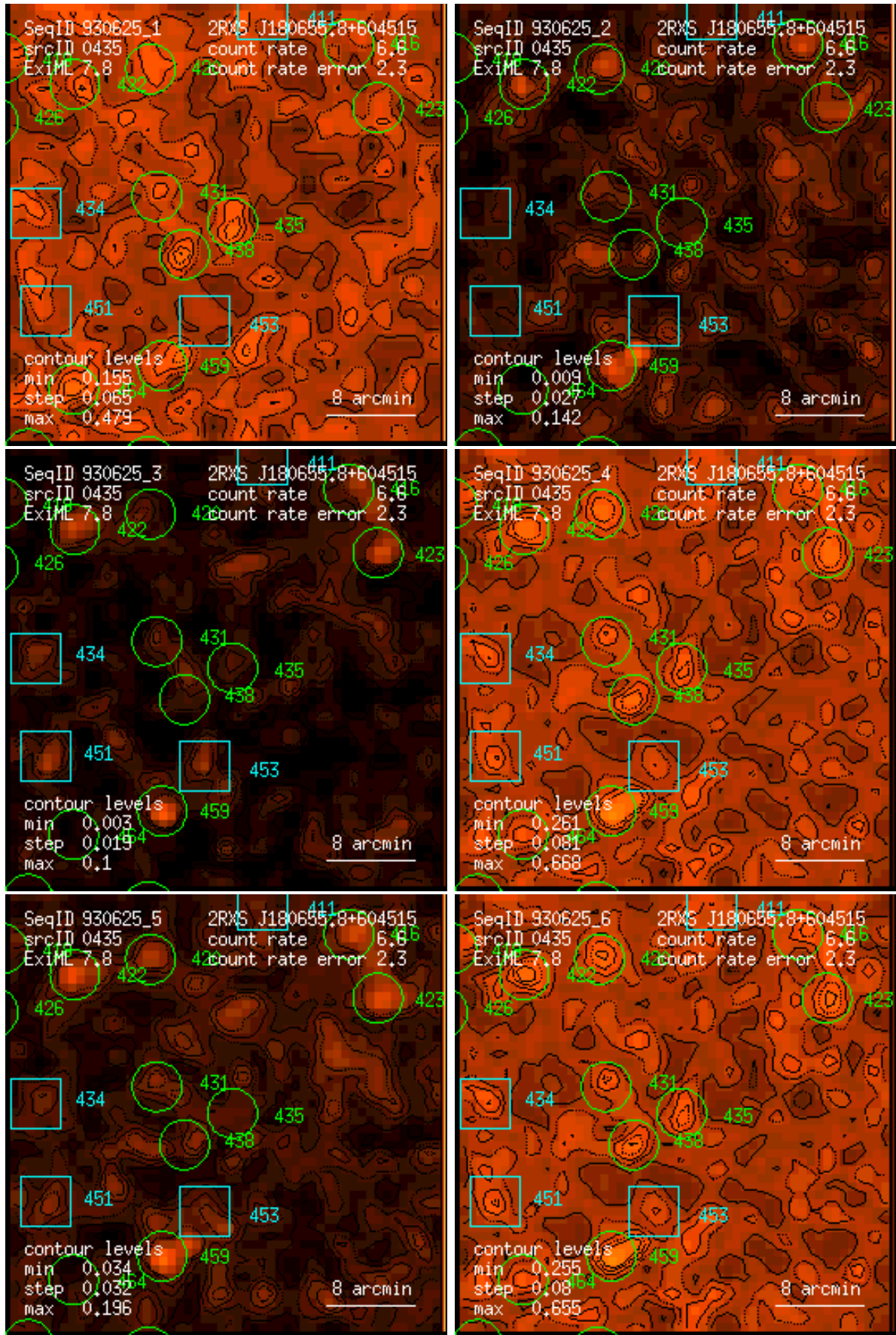
Figure 435: RASS 930625: detection 0435: band rate images, Gaussian filter: (1) PSPC channels 11 – 41, (2) 52 – 90, (3) 91 – 201, (4) 11 – 235, (5) 52 – 201, (6) 11 – 201. Broad band rates in counts/ks. Band rate contour levels in counts/ks/arcmin 2 .
