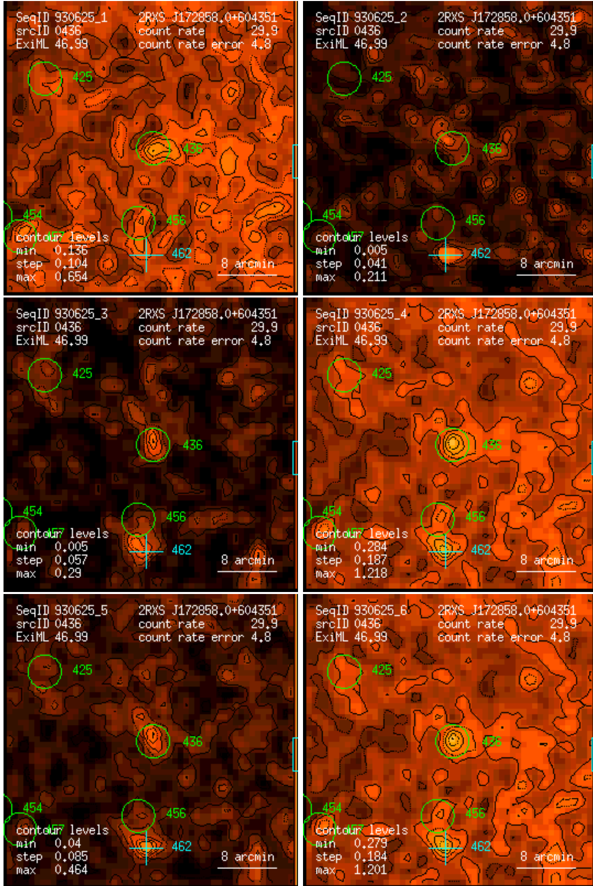
Figure 436: RASS 930625: detection 0436: band rate images, Gaussian filter: (1) PSPC channels 11 – 41, (2) 52 – 90, (3) 91 – 201, (4) 11 – 235, (5) 52 – 201, (6) 11 – 201. Broad band rates in counts/ks. Band rate contour levels in counts/ks/arcmin 2 .
