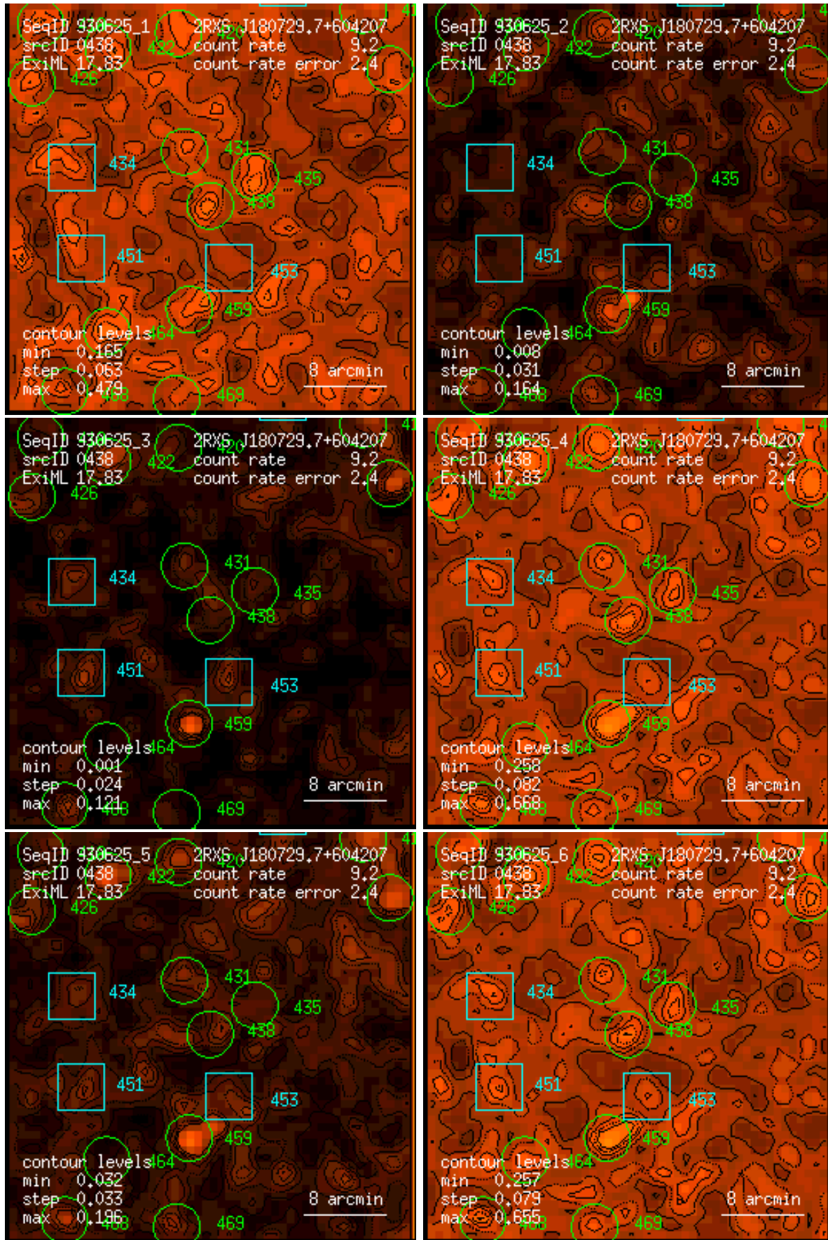
Figure 438: RASS 930625: detection 0438: band rate images, Gaussian filter: (1) PSPC channels 11 – 41, (2) 52 – 90, (3) 91 – 201, (4) 11 – 235, (5) 52 – 201, (6) 11 – 201. Broad band rates in counts/ks. Band rate contour levels in counts/ks/arcmin 2 .
