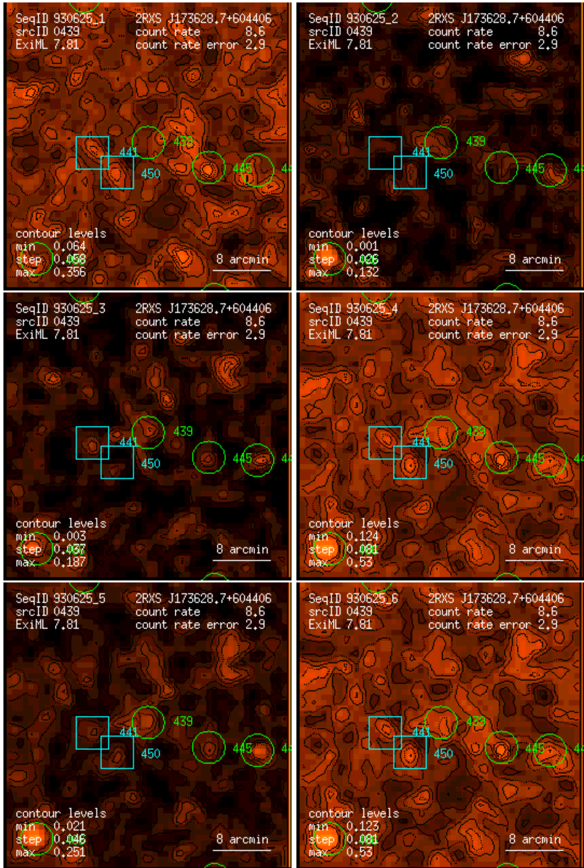
Figure 439: RASS 930625: detection 0439: band rate images, Gaussian filter: (1) PSPC channels 11 – 41, (2) 52 – 90, (3) 91 – 201, (4) 11 – 235, (5) 52 – 201, (6) 11 – 201. Broad band rates in counts/ks. Band rate contour levels in counts/ks/arcmin 2 .
