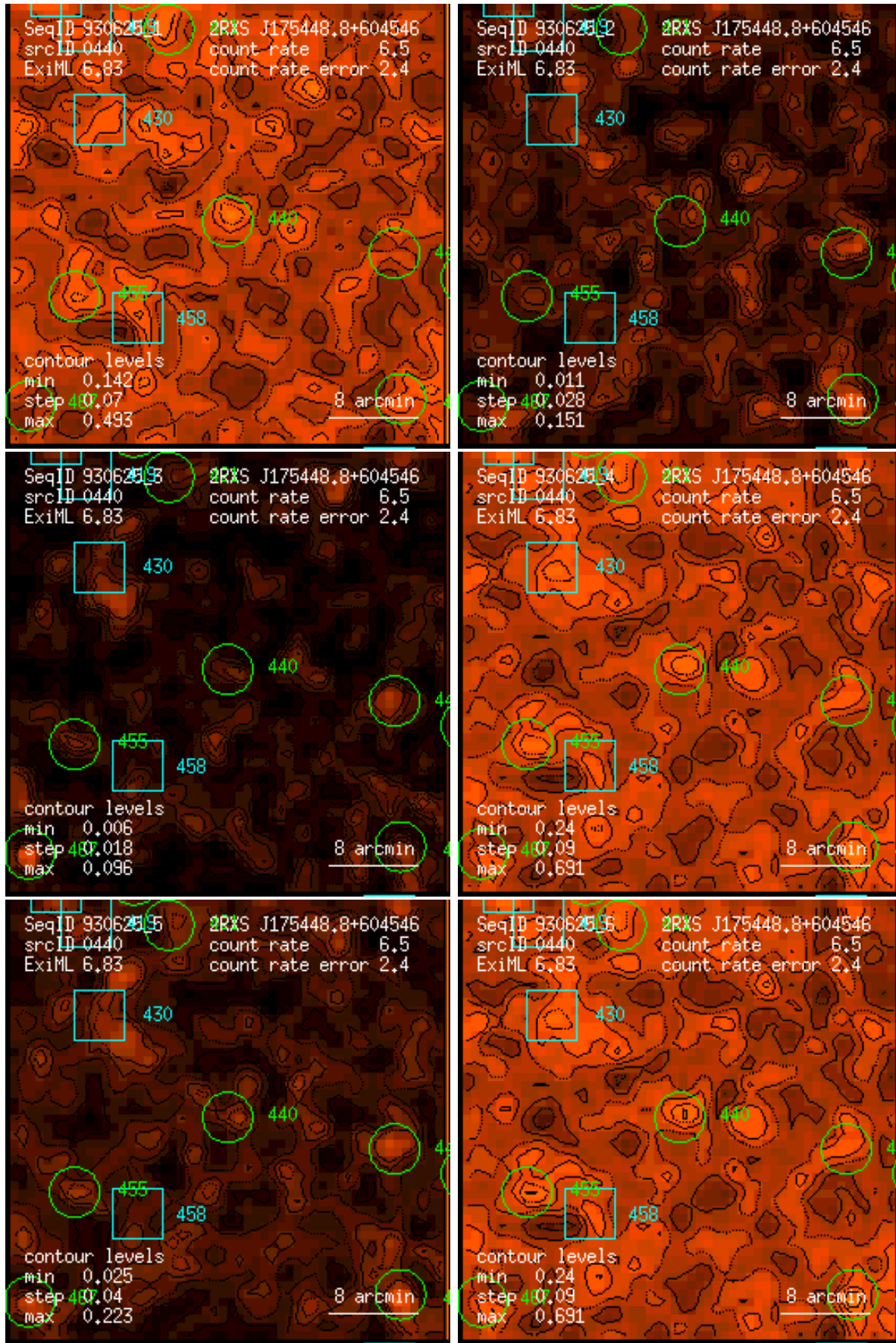
Figure 440: RASS 930625: detection 0440: band rate images, Gaussian filter: (1) PSPC channels 11 – 41, (2) 52 – 90, (3) 91 – 201, (4) 11 – 235, (5) 52 – 201, (6) 11 – 201. Broad band rates in counts/ks. Band rate contour levels in counts/ks/arcmin 2 .
