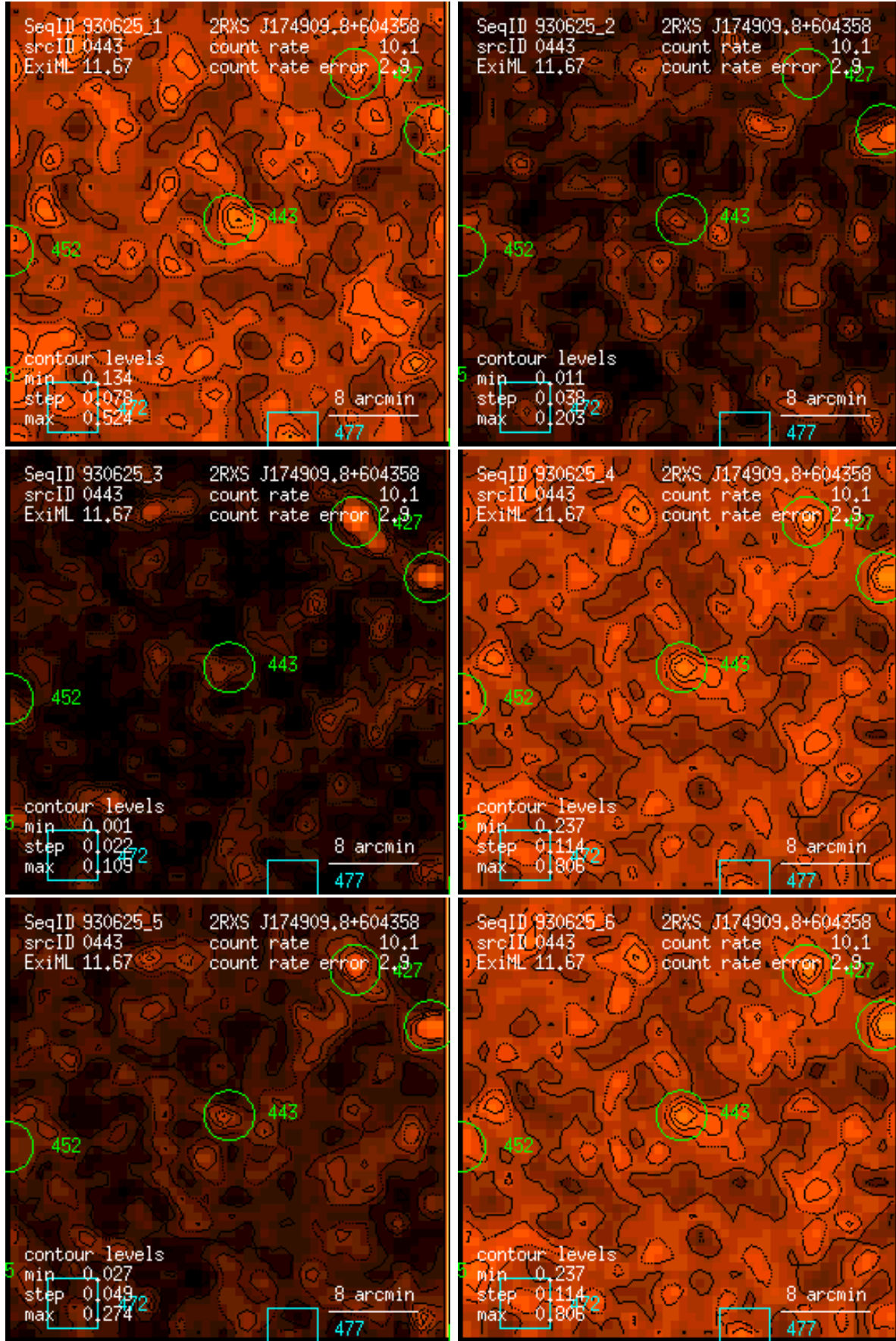
Figure 443: RASS 930625: detection 0443: band rate images, Gaussian filter: (1) PSPC channels 11 – 41, (2) 52 – 90, (3) 91 – 201, (4) 11 – 235, (5) 52 – 201, (6) 11 – 201. Broad band rates in counts/ks. Band rate contour levels in counts/ks/arcmin 2 .
