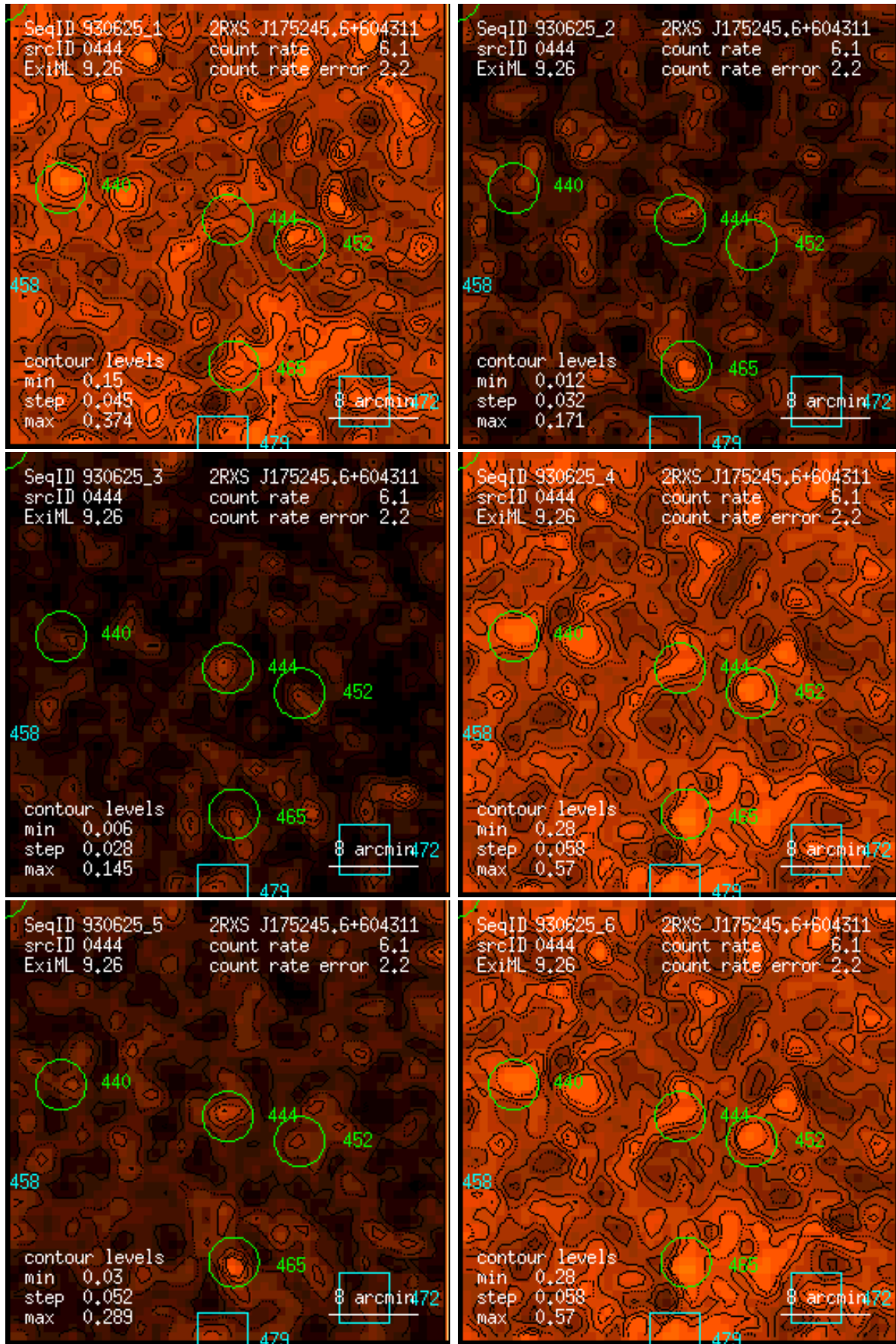
Figure 444: RASS 930625: detection 0444: band rate images, Gaussian filter: (1) PSPC channels 11 – 41, (2) 52 – 90, (3) 91 – 201, (4) 11 – 235, (5) 52 – 201, (6) 11 – 201. Broad band rates in counts/ks. Band rate contour levels in counts/ks/arcmin 2 .
