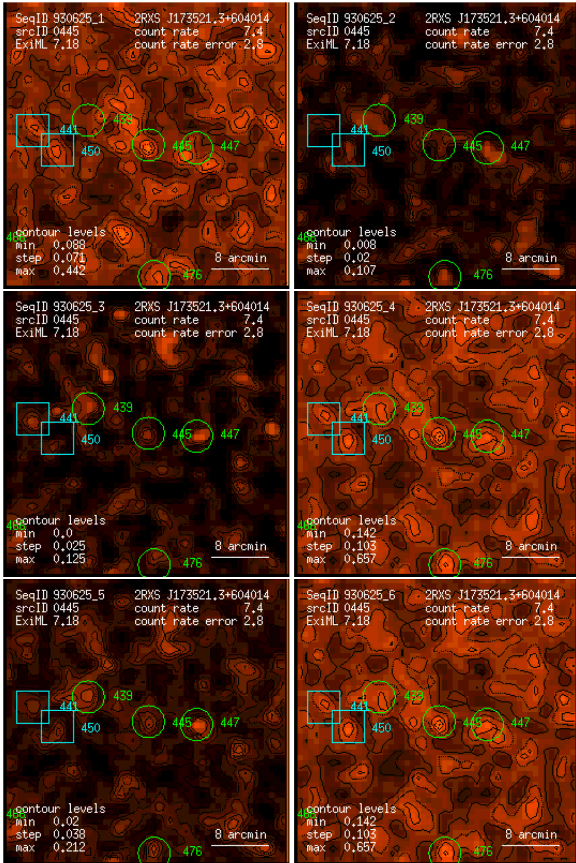
Figure 445: RASS 930625: detection 0445: band rate images, Gaussian filter: (1) PSPC channels 11 – 41, (2) 52 – 90, (3) 91 – 201, (4) 11 – 235, (5) 52 – 201, (6) 11 – 201. Broad band rates in counts/ks. Band rate contour levels in counts/ks/arcmin 2 .
