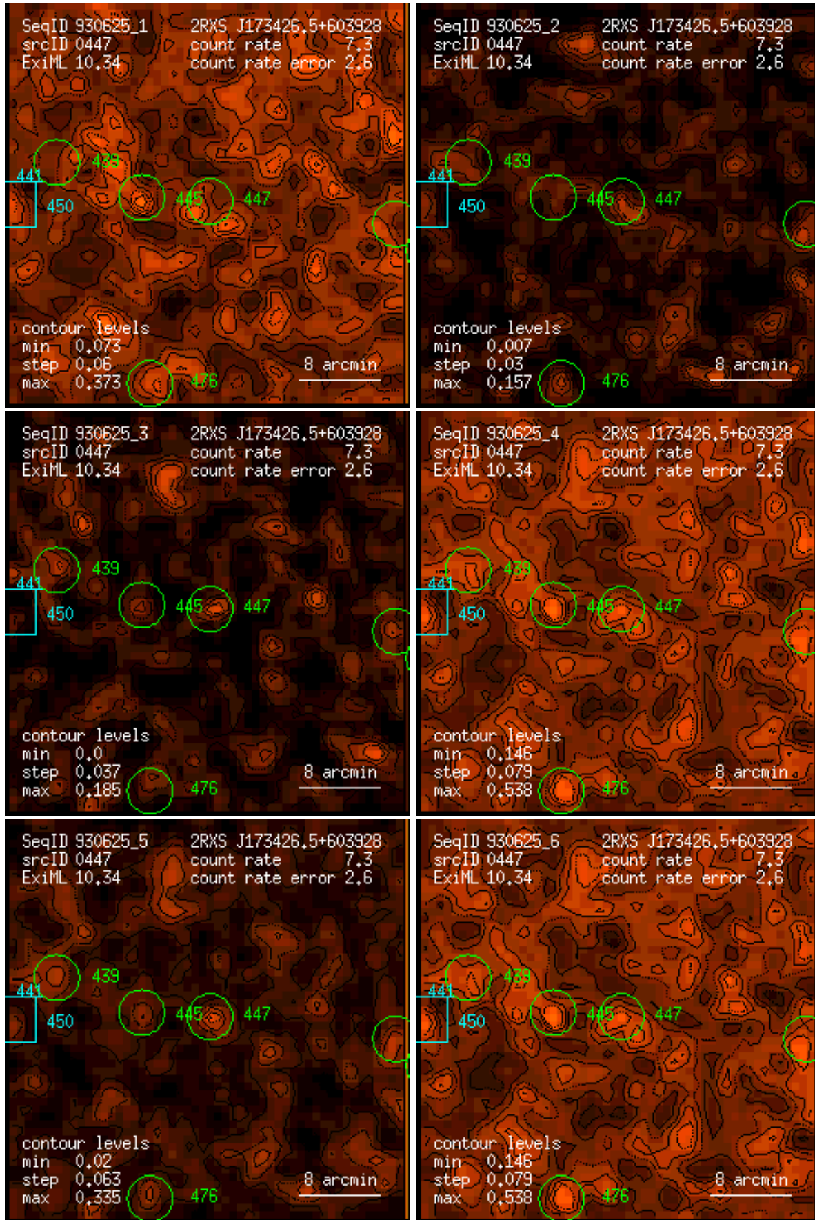
Figure 447: RASS 930625: detection 0447: band rate images, Gaussian filter: (1) PSPC channels 11 – 41, (2) 52 – 90, (3) 91 – 201, (4) 11 – 235, (5) 52 – 201, (6) 11 – 201. Broad band rates in counts/ks. Band rate contour levels in counts/ks/arcmin 2 .
