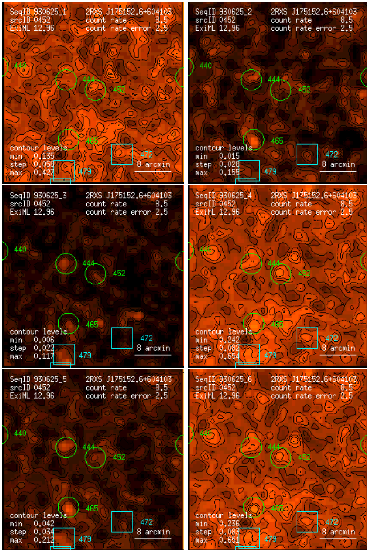
Figure 452: RASS 930625: detection 0452: band rate images, Gaussian filter: (1) PSPC channels 11 – 41, (2) 52 – 90, (3) 91 – 201, (4) 11 – 235, (5) 52 – 201, (6) 11 – 201. Broad band rates in counts/ks. Band rate contour levels in counts/ks/arcmin 2 .
