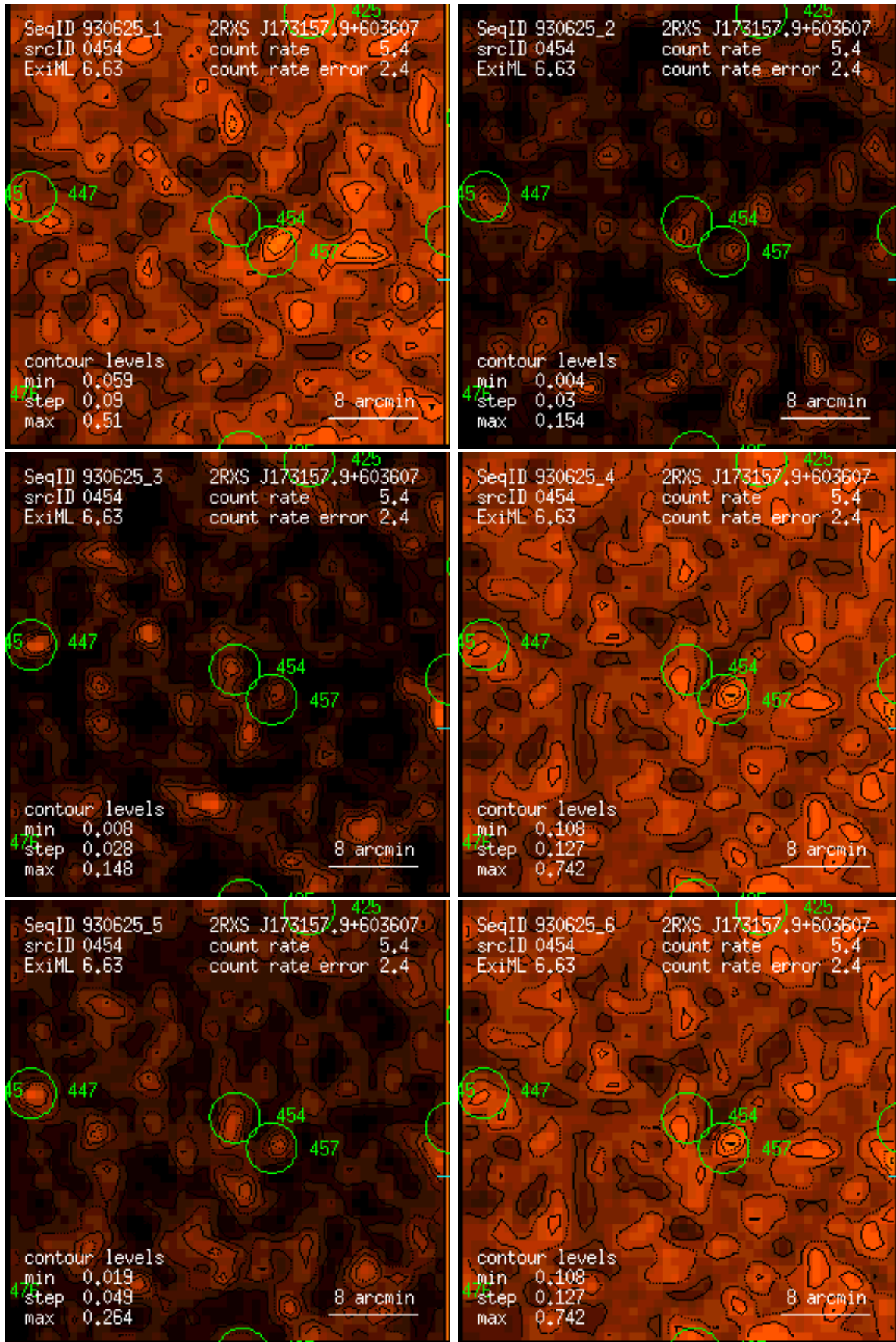
Figure 454: RASS 930625: detection 0454: band rate images, Gaussian filter: (1) PSPC channels 11 – 41, (2) 52 – 90, (3) 91 – 201, (4) 11 – 235, (5) 52 – 201, (6) 11 – 201. Broad band rates in counts/ks. Band rate contour levels in counts/ks/arcmin 2 .
