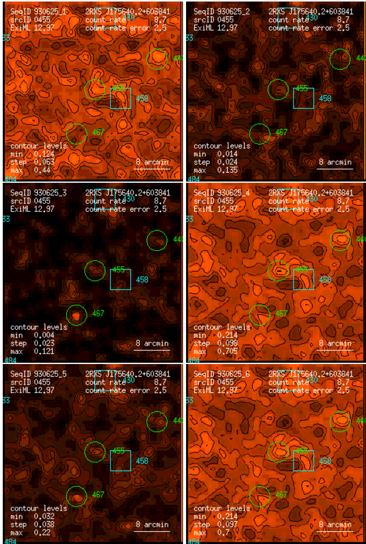
Figure 455: RASS 930625: detection 0455: band rate images, Gaussian filter: (1) PSPC channels 11 – 41, (2) 52 – 90, (3) 91 – 201, (4) 11 – 235, (5) 52 – 201, (6) 11 – 201. Broad band rates in counts/ks. Band rate contour levels in counts/ks/arcmin 2 .
