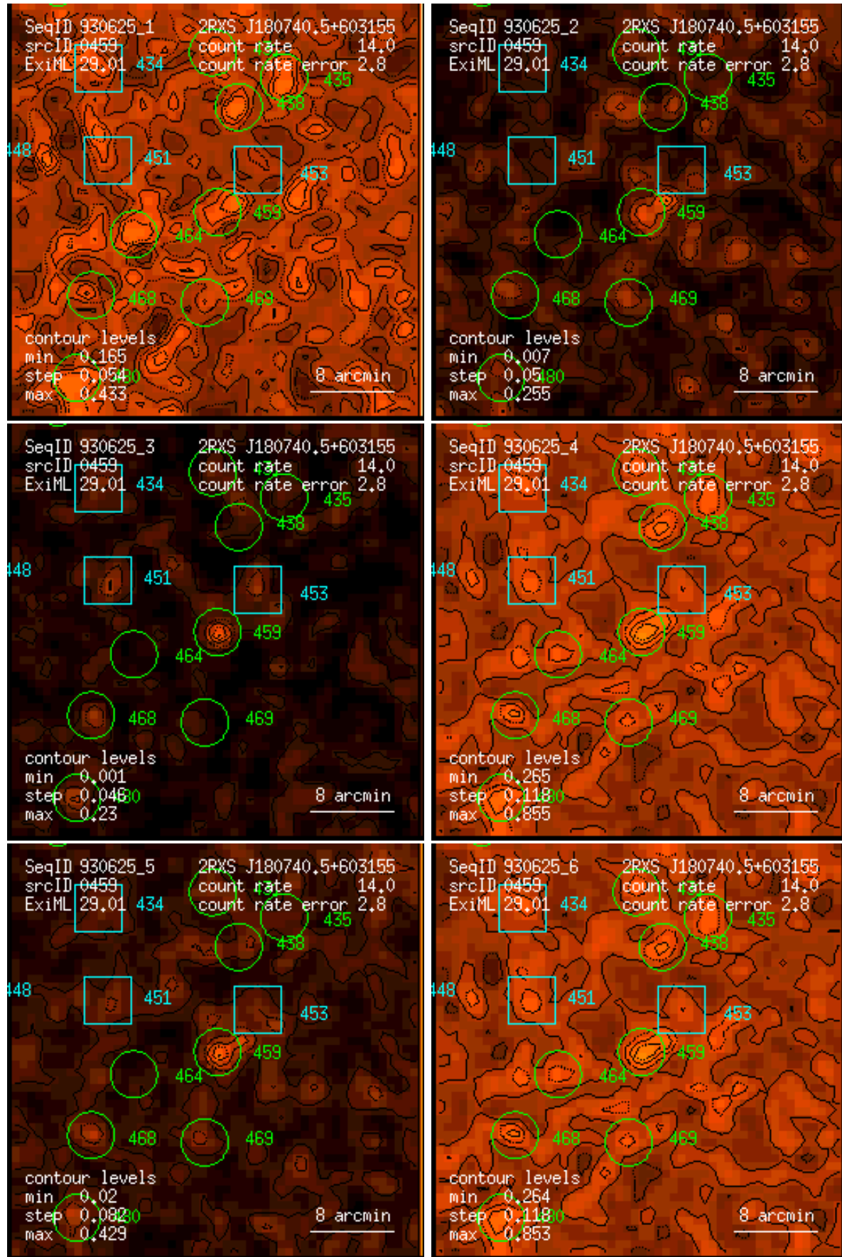
Figure 459: RASS 930625: detection 0459: band rate images, Gaussian filter: (1) PSPC channels 11 – 41, (2) 52 – 90, (3) 91 – 201, (4) 11 – 235, (5) 52 – 201, (6) 11 – 201. Broad band rates in counts/ks. Band rate contour levels in counts/ks/arcmin 2 .
