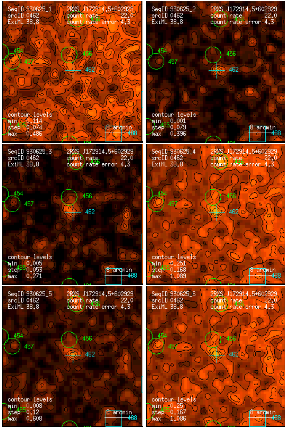
Figure 462: RASS 930625: detection 0462: band rate images, Gaussian filter: (1) PSPC channels 11 – 41, (2) 52 – 90, (3) 91 – 201, (4) 11 – 235, (5) 52 – 201, (6) 11 – 201. Broad band rates in counts/ks. Band rate contour levels in counts/ks/arcmin 2 .
