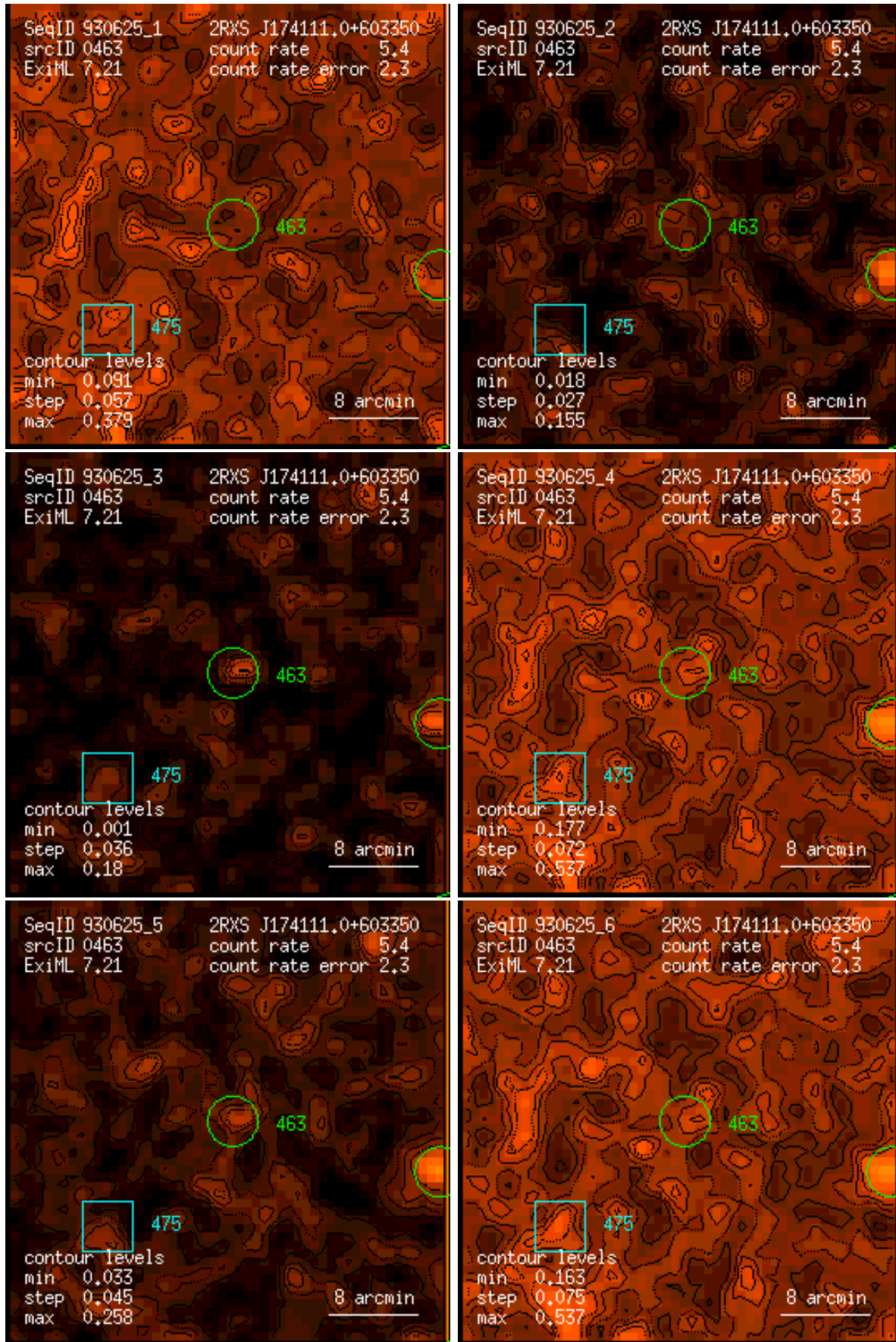
Figure 463: RASS 930625: detection 0463: band rate images, Gaussian filter: (1) PSPC channels 11 – 41, (2) 52 – 90, (3) 91 – 201, (4) 11 – 235, (5) 52 – 201, (6) 11 – 201. Broad band rates in counts/ks. Band rate contour levels in counts/ks/arcmin 2 .
