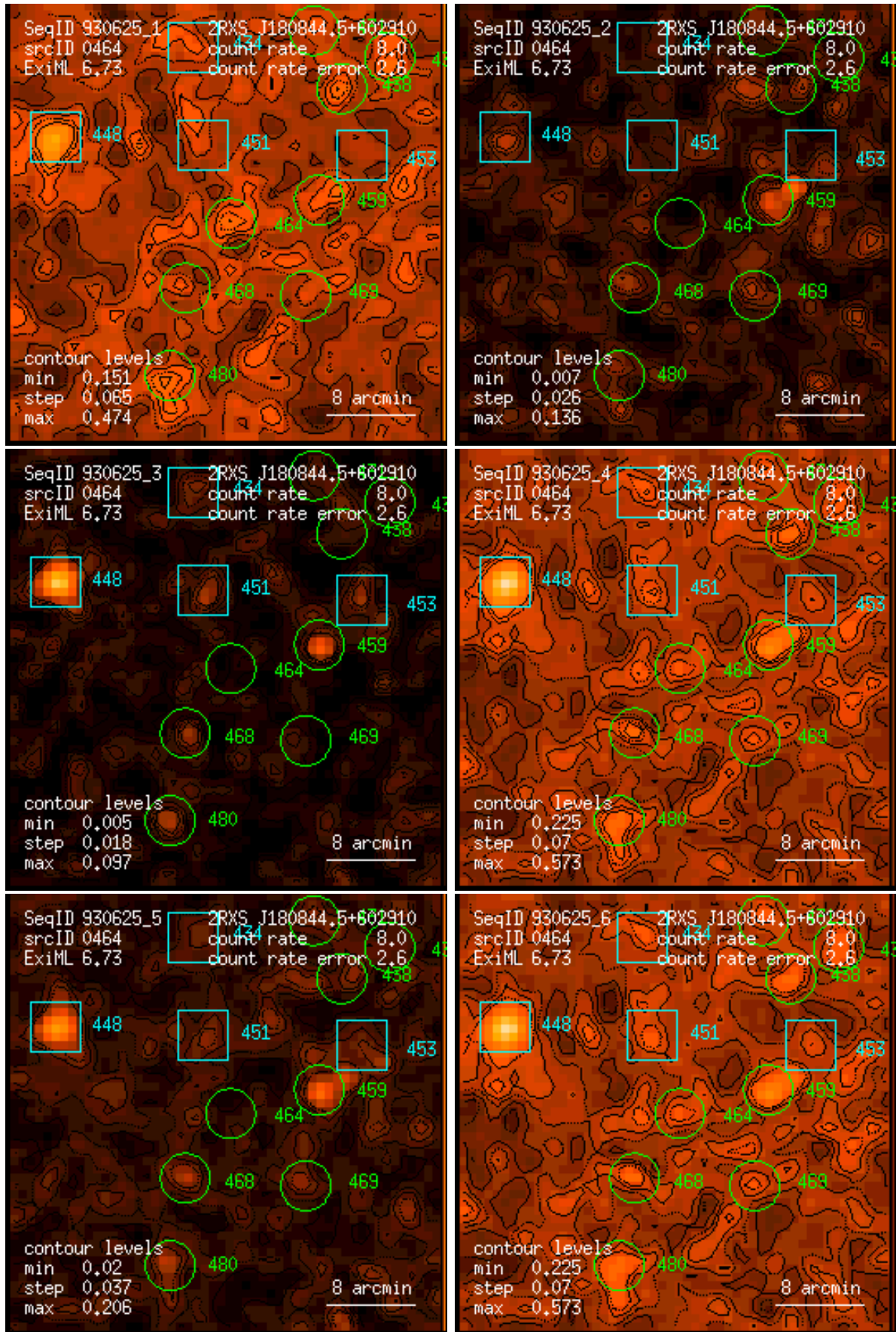
Figure 464: RASS 930625: detection 0464: band rate images, Gaussian filter: (1) PSPC channels 11 – 41, (2) 52 – 90, (3) 91 – 201, (4) 11 – 235, (5) 52 – 201, (6) 11 – 201. Broad band rates in counts/ks. Band rate contour levels in counts/ks/arcmin 2 .
