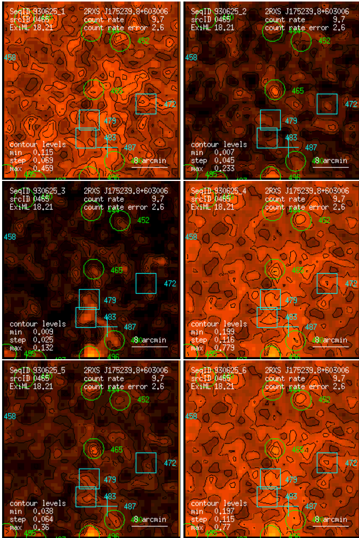
Figure 465: RASS 930625: detection 0465: band rate images, Gaussian filter: (1) PSPC channels 11 – 41, (2) 52 – 90, (3) 91 – 201, (4) 11 – 235, (5) 52 – 201, (6) 11 – 201. Broad band rates in counts/ks. Band rate contour levels in counts/ks/arcmin 2 .
