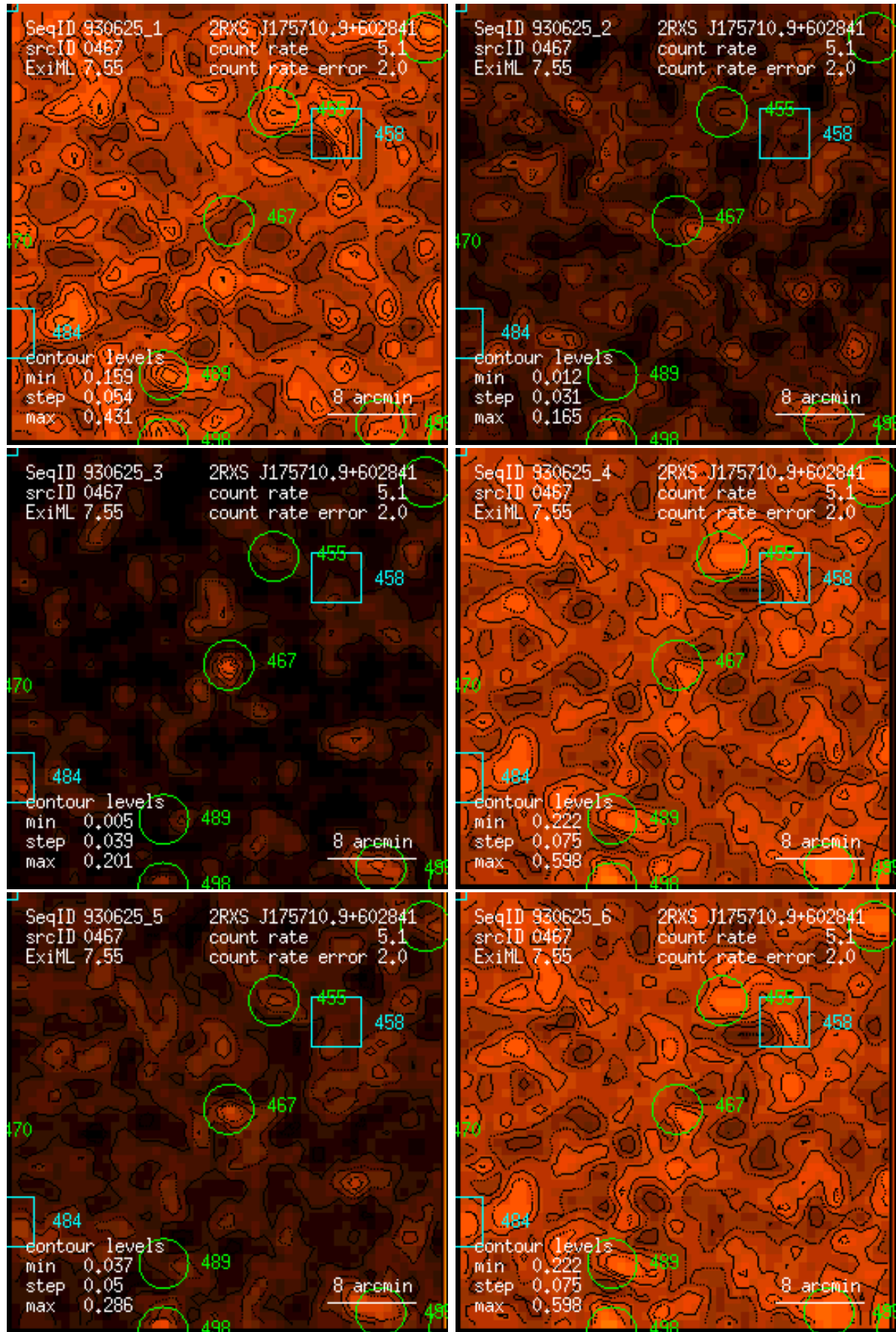
Figure 467: RASS 930625: detection 0467: band rate images, Gaussian filter: (1) PSPC channels 11 – 41, (2) 52 – 90, (3) 91 – 201, (4) 11 – 235, (5) 52 – 201, (6) 11 – 201. Broad band rates in counts/ks. Band rate contour levels in counts/ks/arcmin 2 .
