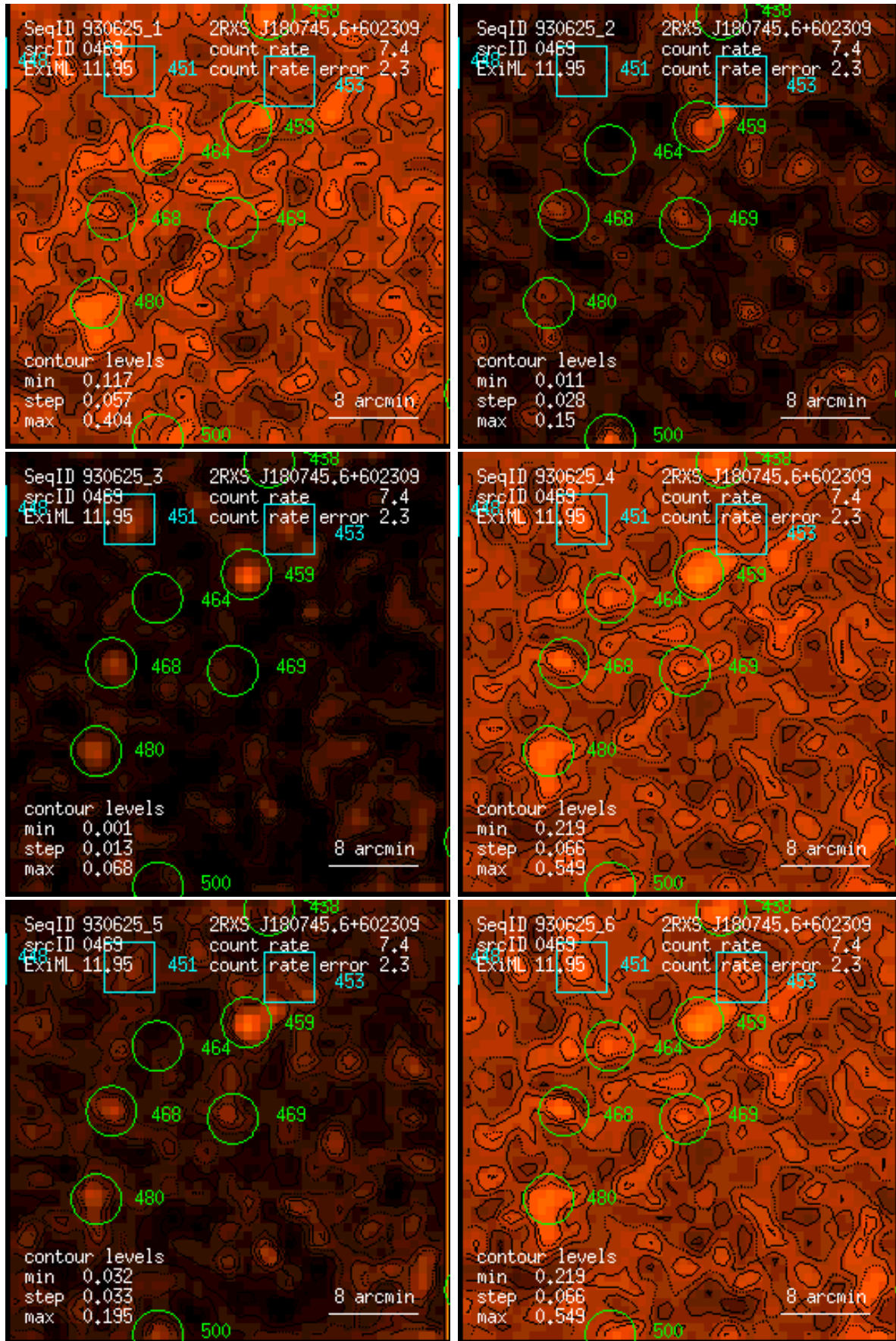
Figure 469: RASS 930625: detection 0469: band rate images, Gaussian filter: (1) PSPC channels 11 – 41, (2) 52 – 90, (3) 91 – 201, (4) 11 – 235, (5) 52 – 201, (6) 11 – 201. Broad band rates in counts/ks. Band rate contour levels in counts/ks/arcmin 2 .
