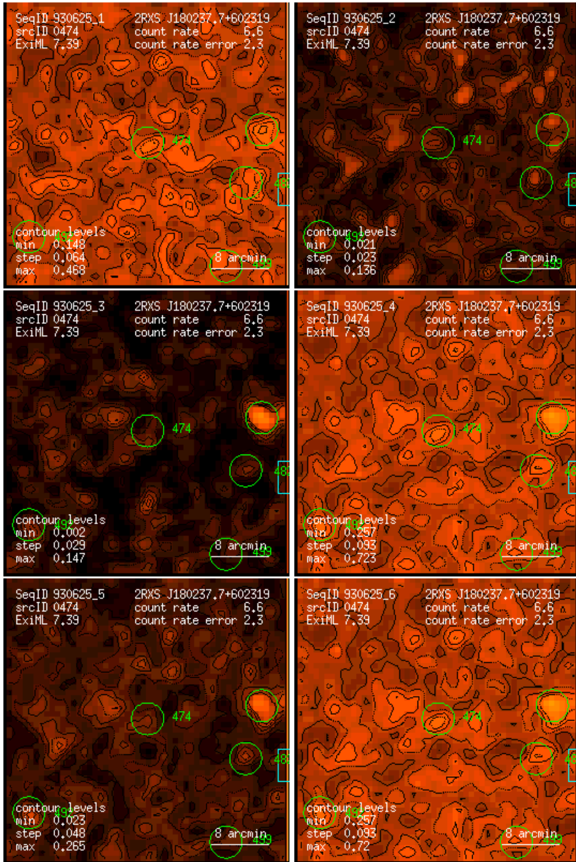
Figure 474: RASS 930625: detection 0474: band rate images, Gaussian filter: (1) PSPC channels 11 – 41, (2) 52 – 90, (3) 91 – 201, (4) 11 – 235, (5) 52 – 201, (6) 11 – 201. Broad band rates in counts/ks. Band rate contour levels in counts/ks/arcmin 2 .
