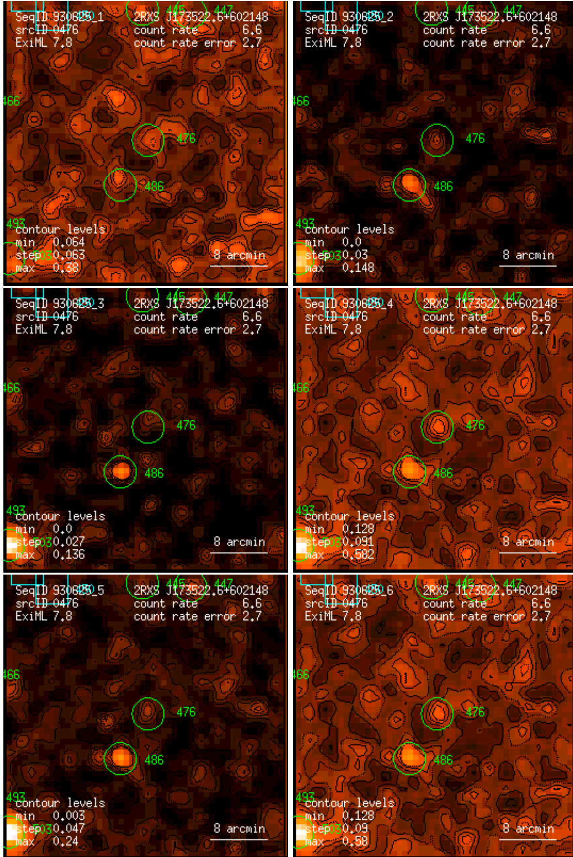
Figure 476: RASS 930625: detection 0476: band rate images, Gaussian filter: (1) PSPC channels 11 – 41, (2) 52 – 90, (3) 91 – 201, (4) 11 – 235, (5) 52 – 201, (6) 11 – 201. Broad band rates in counts/ks. Band rate contour levels in counts/ks/arcmin 2 .
