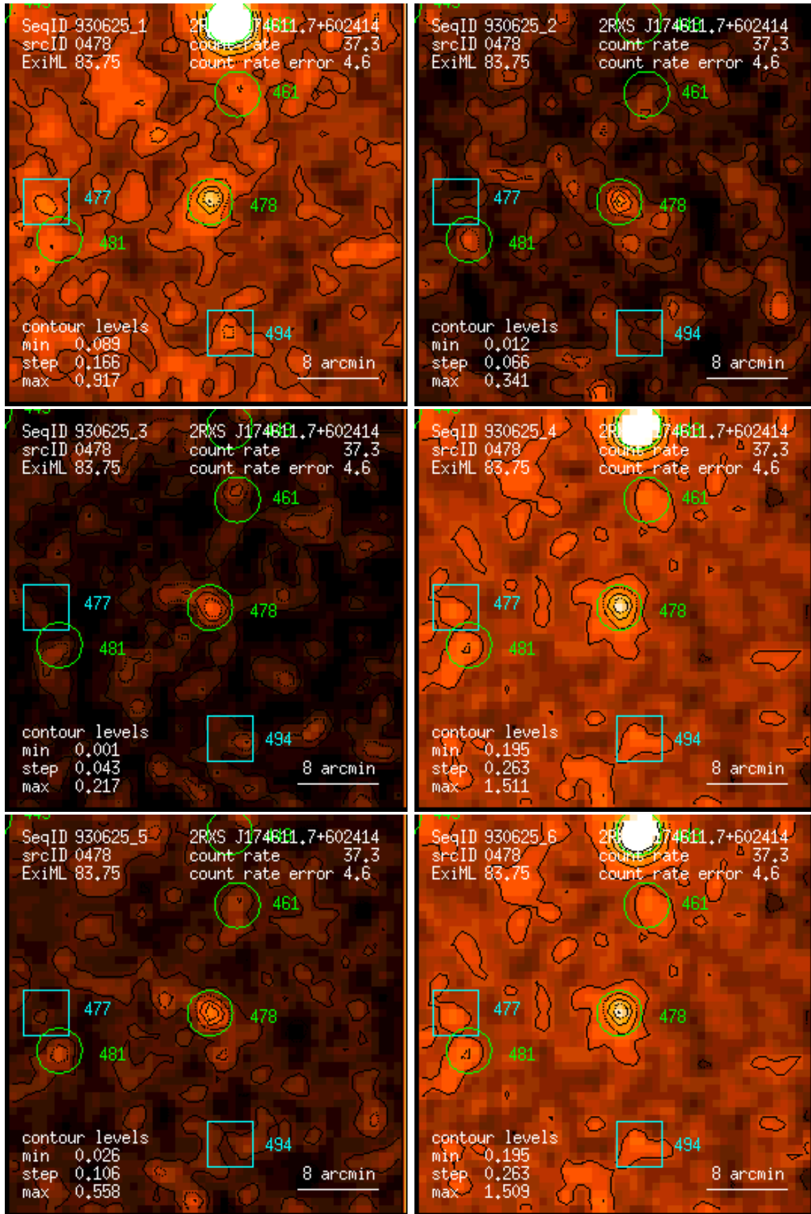
Figure 478: RASS 930625: detection 0478: band rate images, Gaussian filter: (1) PSPC channels 11 – 41, (2) 52 – 90, (3) 91 – 201, (4) 11 – 235, (5) 52 – 201, (6) 11 – 201. Broad band rates in counts/ks. Band rate contour levels in counts/ks/arcmin 2 .
