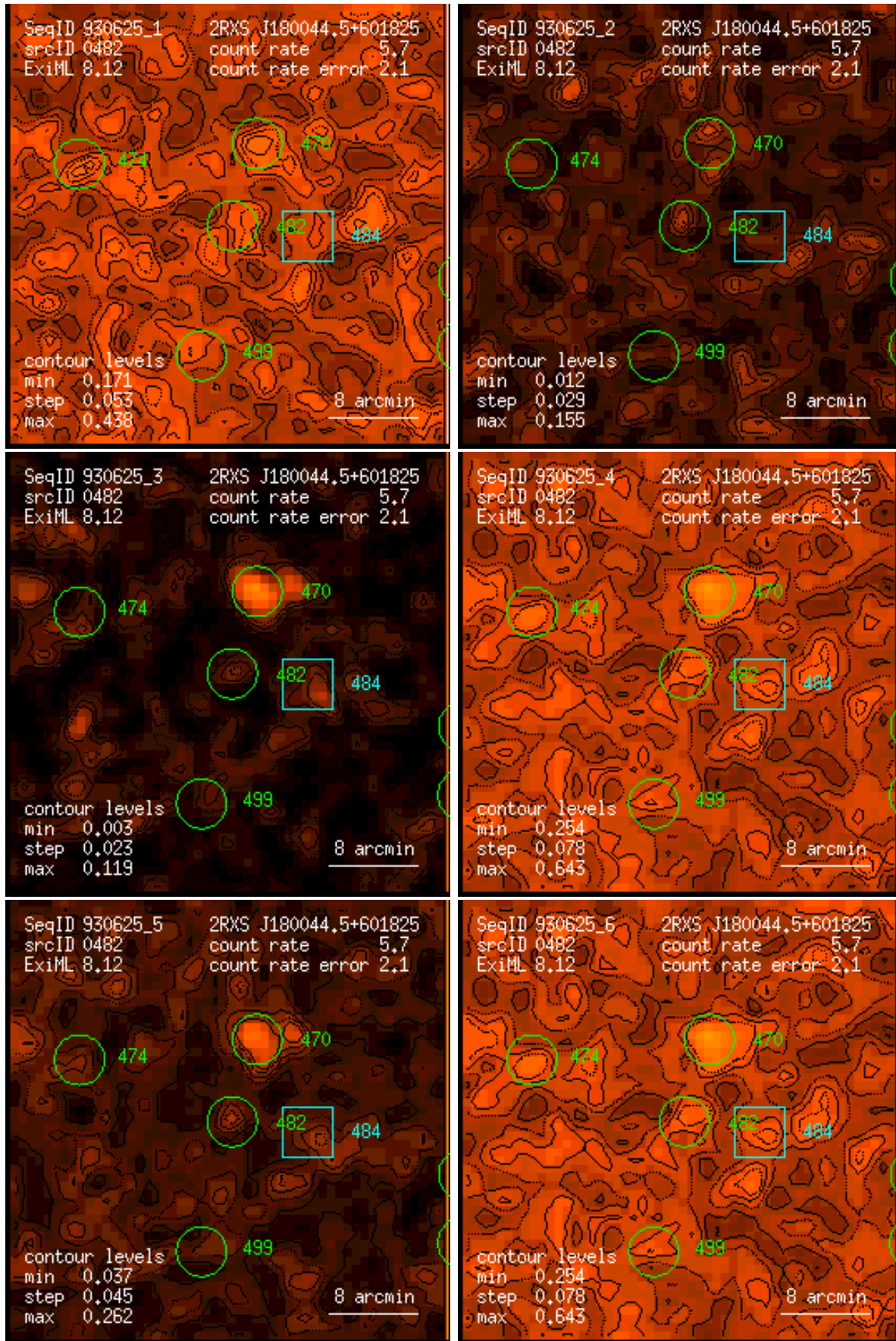
Figure 482: RASS 930625: detection 0482: band rate images, Gaussian filter: (1) PSPC channels 11 – 41, (2) 52 – 90, (3) 91 – 201, (4) 11 – 235, (5) 52 – 201, (6) 11 – 201. Broad band rates in counts/ks. Band rate contour levels in counts/ks/arcmin 2 .
