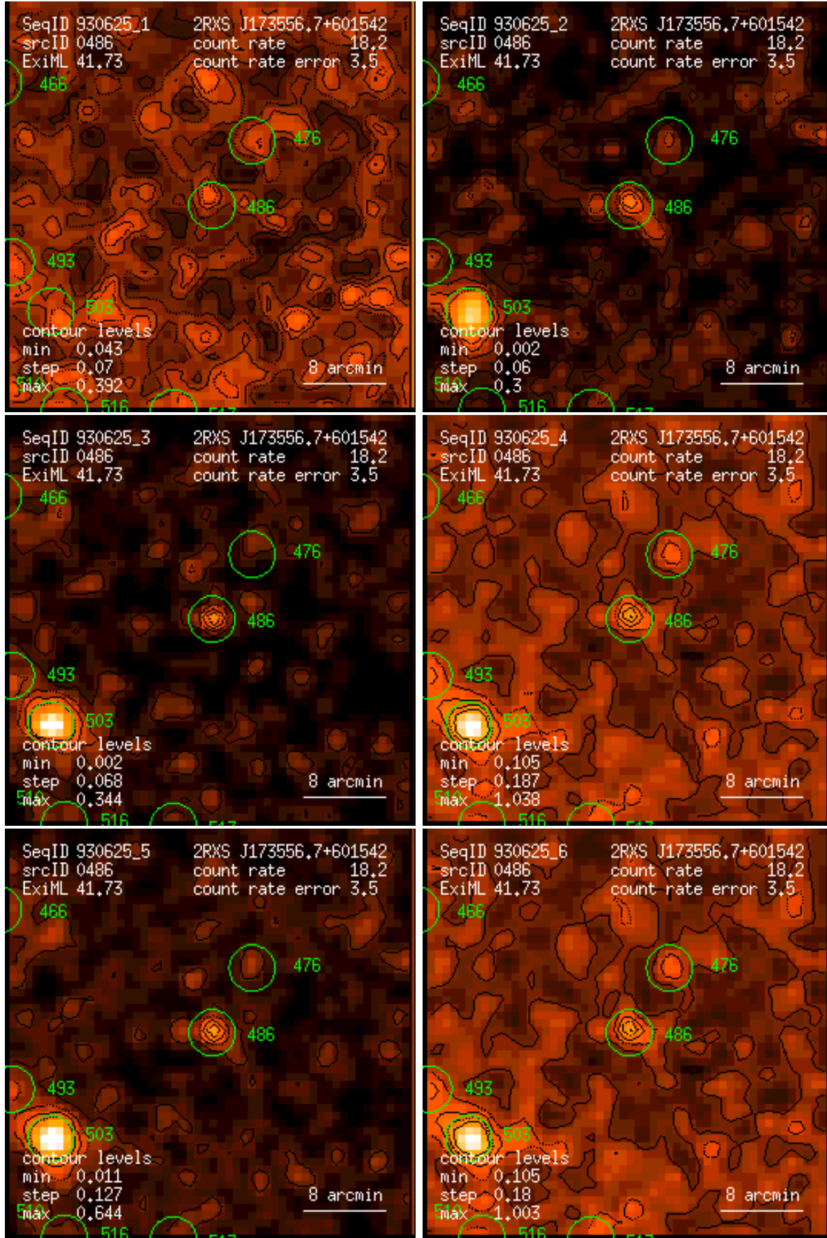
Figure 486: RASS 930625: detection 0486: band rate images, Gaussian filter: (1) PSPC channels 11 – 41, (2) 52 – 90, (3) 91 – 201, (4) 11 – 235, (5) 52 – 201, (6) 11 – 201. Broad band rates in counts/ks. Band rate contour levels in counts/ks/arcmin 2 .
