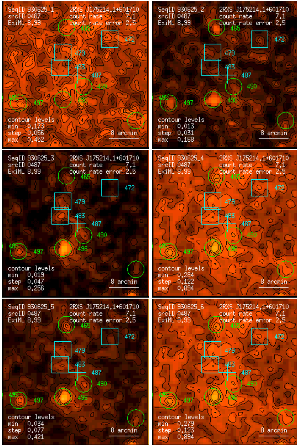
Figure 487: RASS 930625: detection 0487: band rate images, Gaussian filter: (1) PSPC channels 11 – 41, (2) 52 – 90, (3) 91 – 201, (4) 11 – 235, (5) 52 – 201, (6) 11 – 201. Broad band rates in counts/ks. Band rate contour levels in counts/ks/arcmin 2 .
