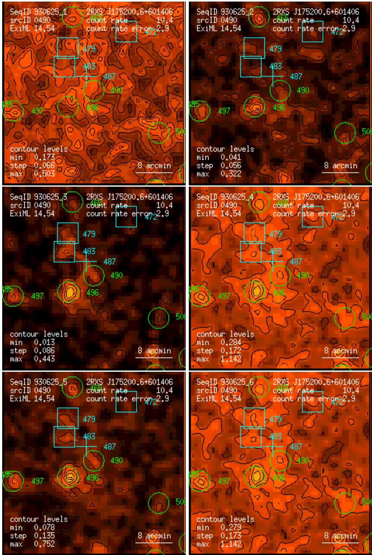
Figure 490: RASS 930625: detection 0490: band rate images, Gaussian filter: (1) PSPC channels 11 – 41, (2) 52 – 90, (3) 91 – 201, (4) 11 – 235, (5) 52 – 201, (6) 11 – 201. Broad band rates in counts/ks. Band rate contour levels in counts/ks/arcmin 2 .
