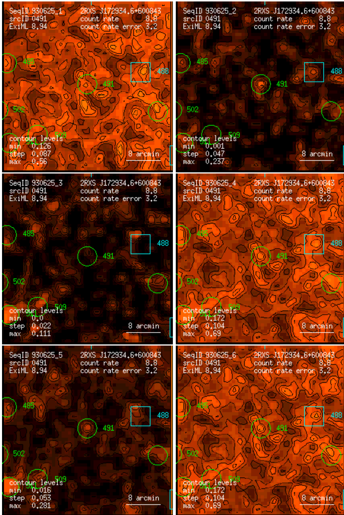
Figure 491: RASS 930625: detection 0491: band rate images, Gaussian filter: (1) PSPC channels 11 – 41, (2) 52 – 90, (3) 91 – 201, (4) 11 – 235, (5) 52 – 201, (6) 11 – 201. Broad band rates in counts/ks. Band rate contour levels in counts/ks/arcmin 2 .
