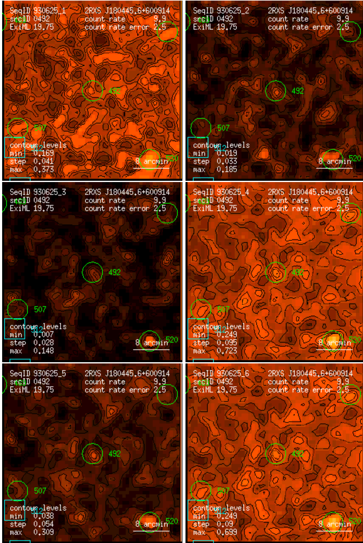
Figure 492: RASS 930625: detection 0492: band rate images, Gaussian filter: (1) PSPC channels 11 – 41, (2) 52 – 90, (3) 91 – 201, (4) 11 – 235, (5) 52 – 201, (6) 11 – 201. Broad band rates in counts/ks. Band rate contour levels in counts/ks/arcmin 2 .
