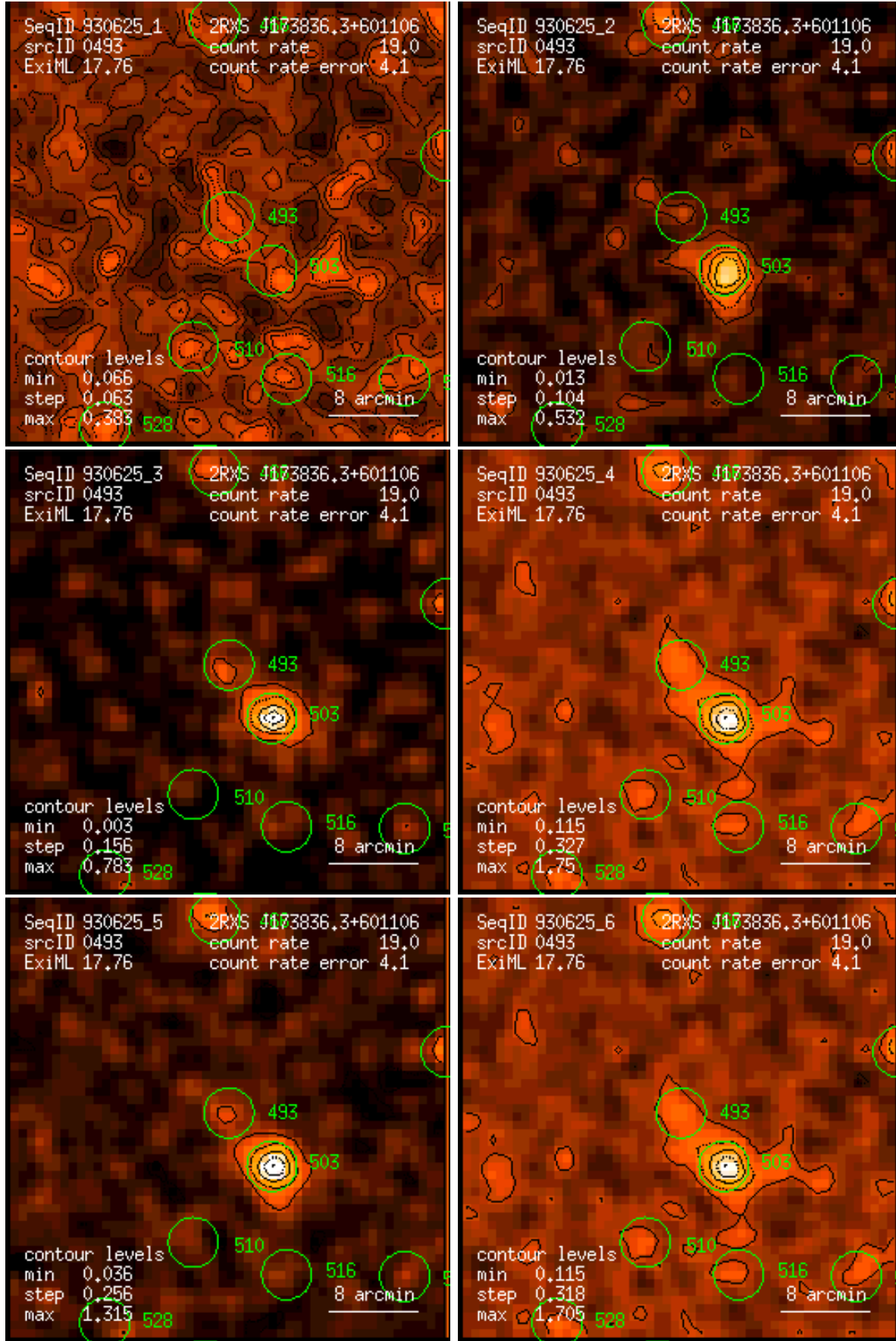
Figure 493: RASS 930625: detection 0493: band rate images, Gaussian filter: (1) PSPC channels 11 – 41, (2) 52 – 90, (3) 91 – 201, (4) 11 – 235, (5) 52 – 201, (6) 11 – 201. Broad band rates in counts/ks. Band rate contour levels in counts/ks/arcmin 2 .
