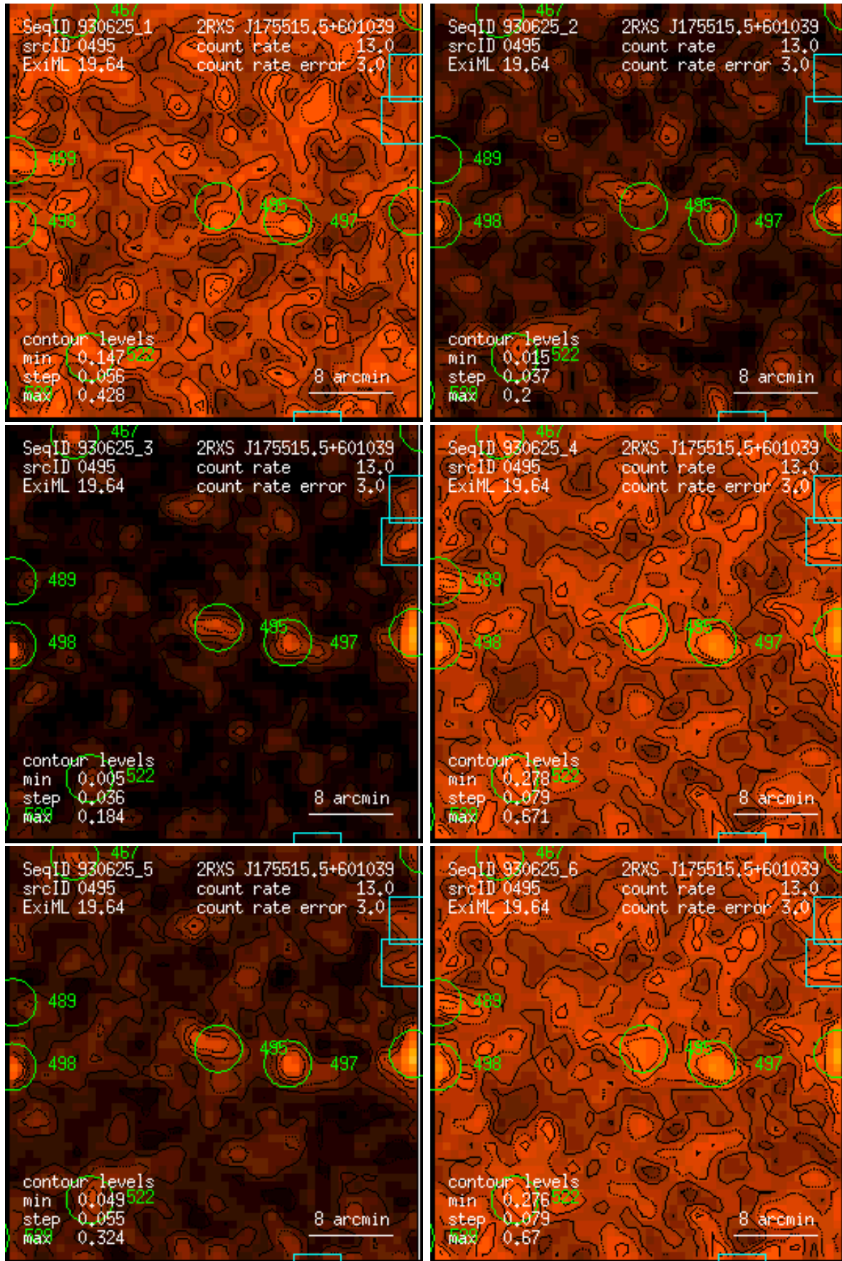
Figure 495: RASS 930625: detection 0495: band rate images, Gaussian filter: (1) PSPC channels 11 – 41, (2) 52 – 90, (3) 91 – 201, (4) 11 – 235, (5) 52 – 201, (6) 11 – 201. Broad band rates in counts/ks. Band rate contour levels in counts/ks/arcmin 2 .
