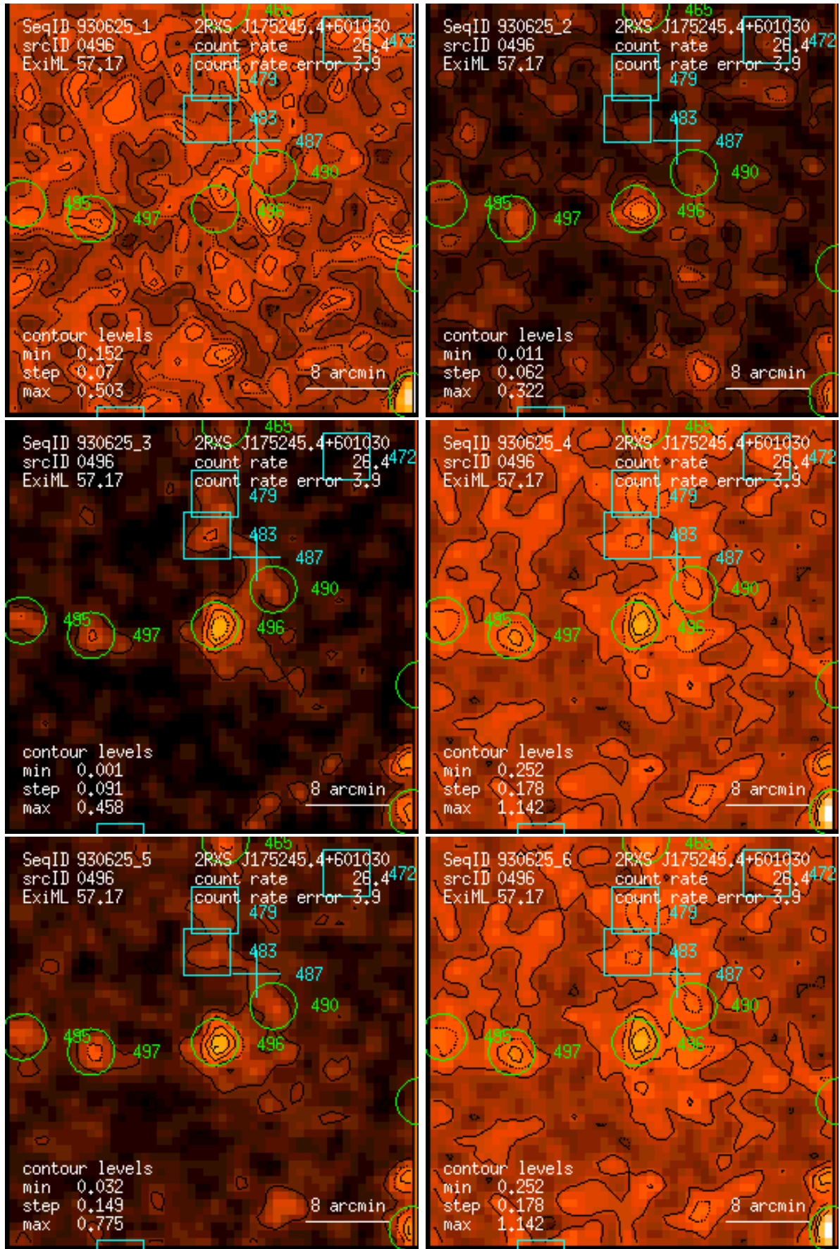
Figure 496: RASS 930625: detection 0496: band rate images, Gaussian filter: (1) PSPC channels 11 – 41, (2) 52 – 90, (3) 91 – 201, (4) 11 – 235, (5) 52 – 201, (6) 11 – 201. Broad band rates in counts/ks. Band rate contour levels in counts/ks/arcmin 2 .
